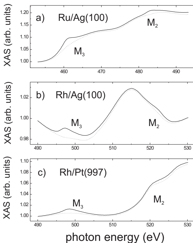
FIG. 1. M_{3,2} XAS spectra of (a) Ru (0.22 ML), (b) Rh (0.09 ML) deposited on Ag(100), and (c) Rh (0.12 ML) on Pt(997) at T = 5 K. The spectra were normalized to unity at the M_3 pre-edge energies. The background XAS measured prior to deposition on pristine Ag and Pt substrates is represented by dotted lines.
