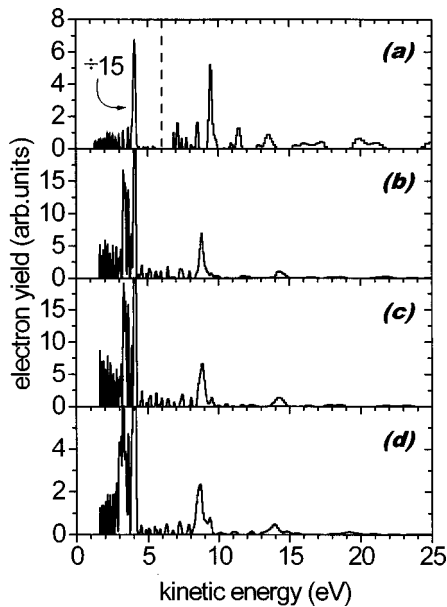
FIG. 2. ATI spectra of Ar for a selection of intensities. (a) 8.1 \times 10^{13} \text{ W cm}^{-2} —the part left of the dashed line has been reduced by a factor of 15 to show the sharp feature in the first photoelectron peak, (b) 1.5 \times 10^{14} \text{ W cm}^{-2} , (c) 2.1 \times 10^{14} \text{ W cm}^{-2} , (d) 2.3 \times 10^{15} \text{ W cm}^{-2} .
