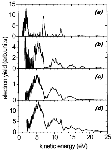
FIG. 1. ATI spectra of Ne for a selection of intensities. (a) 4.8 \times 10^{14} \text{ W cm}^{-2} , (b) 8.6 \times 10^{14} \text{ W cm}^{-2} , (c) 1.1 \times 10^{15} \text{ W cm}^{-2} , (d) 2.4 \times 10^{15} \text{ W cm}^{-2} .
