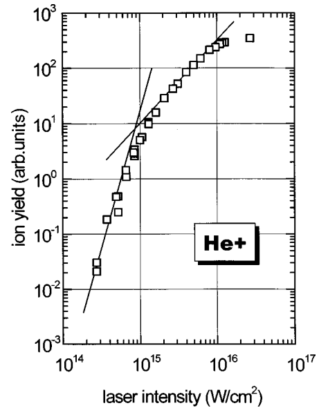
FIG. 3. Ion yield curve for He. To guide the eye, straight lines with slopes of 5 and \frac{3}{2} are inserted.
