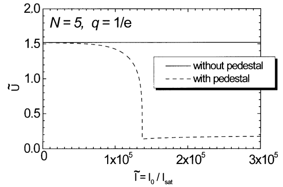
FIG. 10. The effect of a pedestal. The curve shows the normalized ponderomotive shift \tilde{U}_{1/e} as a function of normalized intensity \tilde{I} for a hyperbolic secant squared pulse with a FWHM of 500 fs, calculated for N=5 and q=1/e . Solid line: no pedestal, dashed line: with pedestal.
