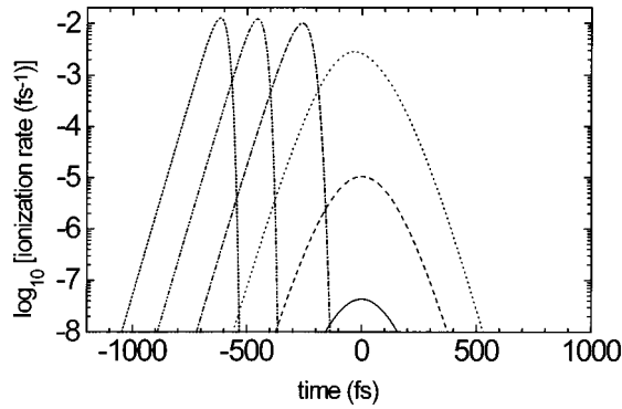
FIG. 7. Typical multiphoton ionization rate curves for a five-photon process with \sigma_{(5)} = 1.0 \times 10^{-152} \text{ cm}^{10} \text{ s}^4 , for a hyperbolic secant squared pulse with a FWHM of 500 fs ( I_{\text{sat}} = 6.8 \times 10^{14} \text{ W cm}^{-2} ), and for a photon energy \hbar\omega = 4.99 \text{ eV} . Rate curves are shown for intensities that are 0.1 (—), 0.3 (---), 1 (·····), 3 (-·-·-·), 10 (- - - - -), and 30 (·-·-·-·) times the saturation intensity.
