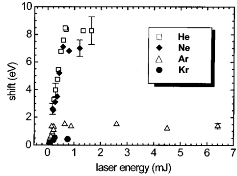
FIG. 6. Measured ponderomotive shifts as a function of laser energy for He, Ne, Ar, and Kr. Some typical error bars are shown.
