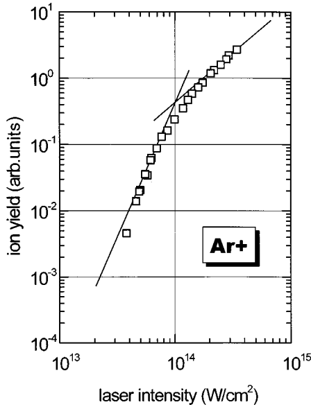
FIG. 5. Ion yield curve for Ar. To guide the eye, straight lines with slopes of 4 and \frac{3}{2} are inserted.
