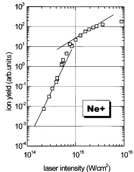
FIG. 4. Ion yield curve for Ne. To guide the eye, straight lines with slopes of 5 and \frac{3}{2} are inserted.
