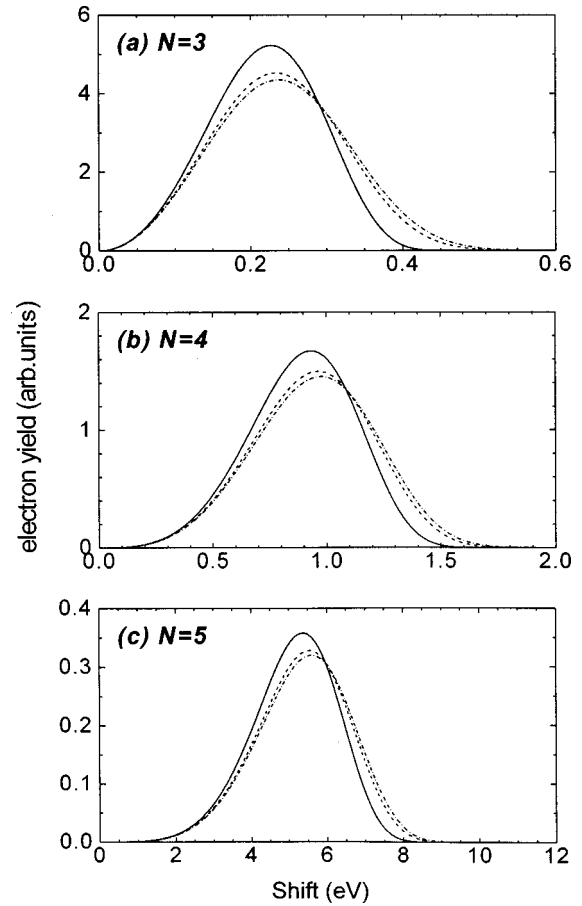
FIG. 8. Calculated electron yield curves Y(U_p) as a function of the ponderomotive shift U_p for intensities above the saturation intensity. All curves were calculated for a hyperbolic secant squared pulse with a FWHM of 500 fs and for a photon energy \hbar\omega = 4.99 \text{ eV} . The following numeric values were used for the generalized cross sections: (a) N=3 , \sigma_{(3)} = 1.0 \times 10^{-82} \text{ cm}^6 \text{ s}^2 , or I_{\text{sat}} = 2.6 \times 10^{13} \text{ W cm}^{-2} ; (b) N=4 , \sigma_{(4)} = 1.0 \times 10^{-116} \text{ cm}^8 \text{ s}^3 , or I_{\text{sat}} = 1.1 \times 10^{14} \text{ W cm}^{-2} ; (c) N=5 , \sigma_{(5)} = 1.0 \times 10^{-152} \text{ cm}^{10} \text{ s}^4 , or I_{\text{sat}} = 6.8 \times 10^{14} \text{ W cm}^{-2} . Electron yield curves are shown for intensities that are 3 (—), 10 (·····), and 100 (-·-·-·) times the saturation intensity.
