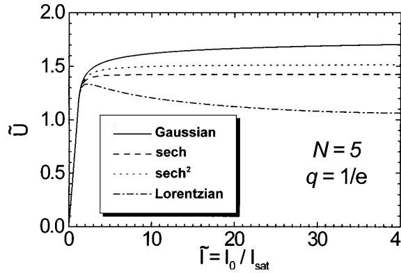
FIG. 9. Calculated curves of the normalized ponderomotive shift \tilde{U}_{1/e} as a function of normalized intensity \tilde{I} for four different laser temporal pulse shapes: Gaussian, hyperbolic secant, hyperbolic secant squared, and Lorentzian. The curves were calculated for N=5 and q=1/e . The FWHM of all four laser pulse shapes is 500 fs.
