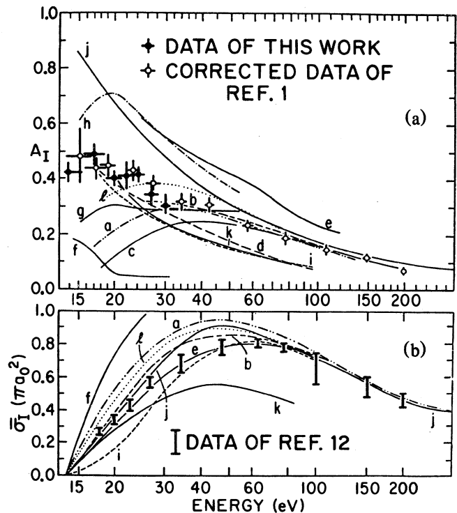
FIG. 1. (a) Measured values of A_I as a function of incident electron energy. Vertical error bars include statistical and systematic uncertainties. Horizontal bars indicate full width at half maximum energy spread of the electron beam. The theoretical curves are obtained from information in the following references using the procedure given in Ref. 2: Curves a, g, and h, Ref. 4; b and e, Ref. 5; c, Ref. 6; d and i, Ref. 7; f, Ref. 8; j, Ref. 9; k, Ref. 10; l, Ref. 11. (b) Experimental values of \bar{\sigma}_1 obtained by other investigators; vertical bars indicate the spread of the measurements. Theoretical curves are from references given above.
