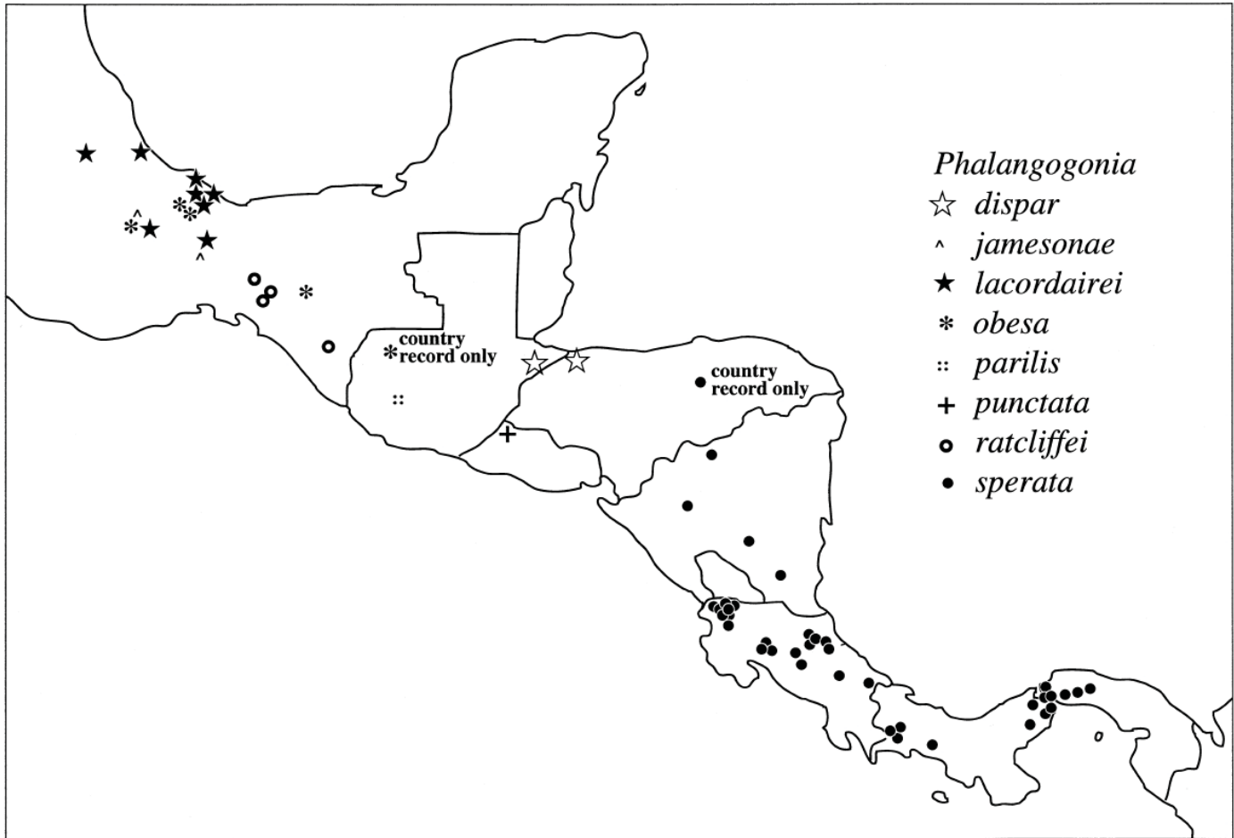
Fig. 4. Distribution of Phalangogonia species in Central America.
