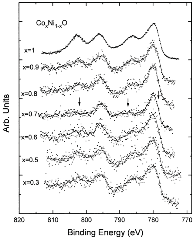
Figure 8. Cobalt 2p XPS for the \text{Co}_x\text{Ni}_{1-x}\text{O} solid solutions over the range of bulk x values. Arrows at the top of the x = 0.7 spectrum emphasize spectral changes described in the text. Discrete points represent actual data and the solid lines are three point smoothed fits to the data.
