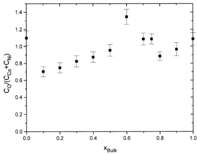
Figure 3. Atomic ratio of oxygen to total metal (Co+Ni) as a function of the bulk x value, obtained from integrated Auger spectra as described in the text. Error bars represent uncertainty in determining peak intensities in the peak fitting procedure.
