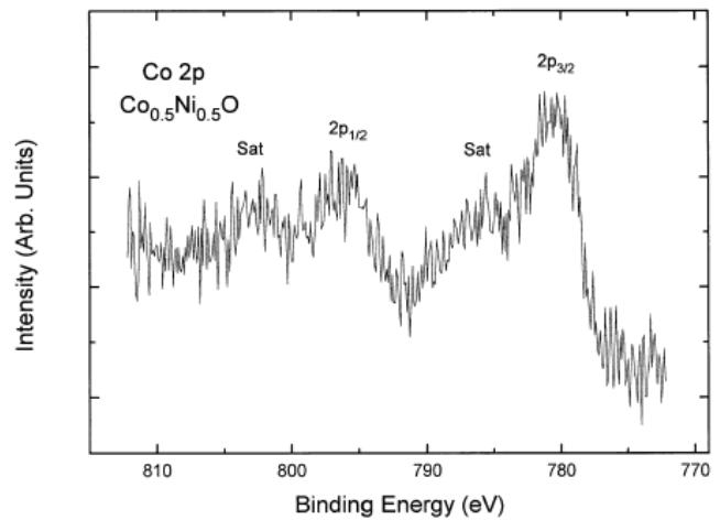
Figure 4. Cobalt 2p XPS for the \text{Co}_{0.5}\text{Ni}_{0.5}\text{O} solid solution.
