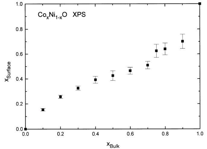
Figure 9. Surface ( x_{\text{surface}} ) cobalt concentration as a function of the bulk ( x_{\text{bulk}} ) value, measured by XPS. Error bars represent uncertainty in determining peak intensities in the peak fitting procedure.
