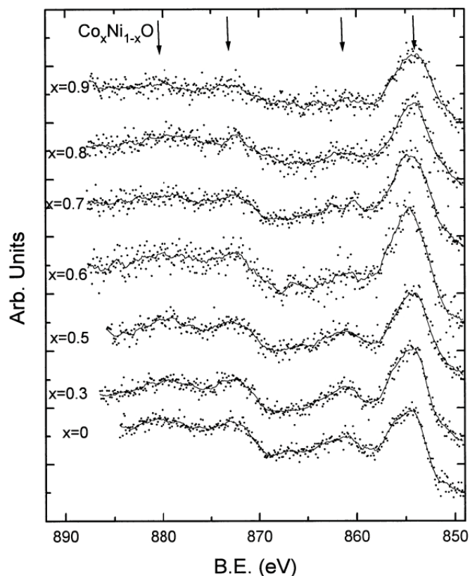
Figure 7. Nickel 2p XPS for the \text{Co}_x\text{Ni}_{1-x}\text{O} solid solutions over the range of bulk x values. Arrows at the top of the x = 0.9 spectrum emphasize spectral changes described in the text. Discrete points represent actual data and the solid lines are three point smoothed fits to the data.
