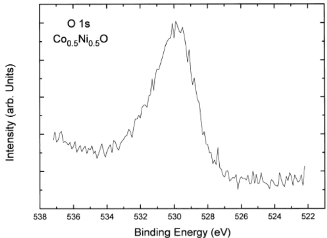
Figure 6. Oxygen 1s XPS for the \text{Co}_{0.5}\text{Ni}_{0.5}\text{O} solid solution.
