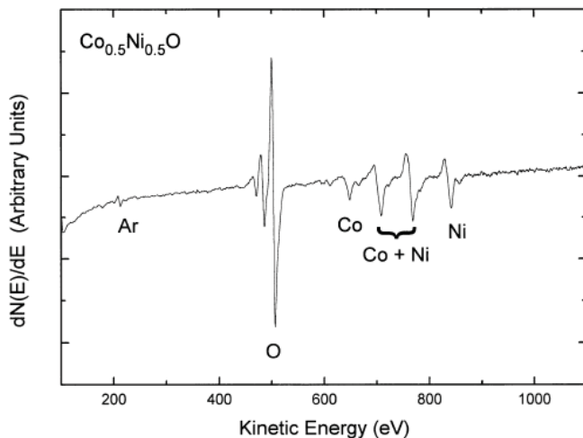
Figure 1. Differential Auger spectrum of the \text{Co}_{0.5}\text{Ni}_{0.5}\text{O} solid solution. The argon impurity results from a brief sputter treatment described in the text. The cobalt L_3M_{2,3}V and L_3M_{2,3}M_{2,3} transitions overlap with those of the nickel L_3VV and L_3M_{2,3}V , as labeled and described more fully in the text.
