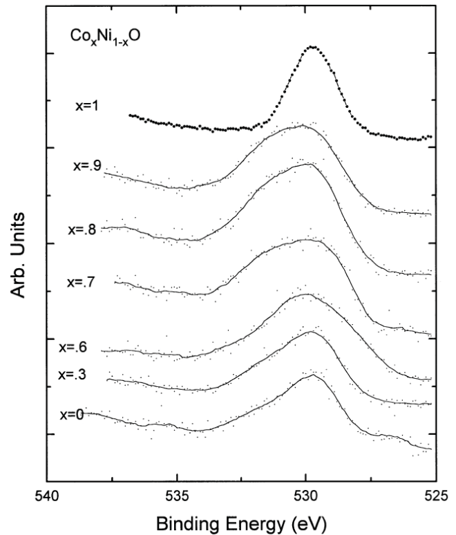
Figure 10. Oxygen 1s XPS for the \text{Co}_x\text{Ni}_{1-x}\text{O} solid solutions over the range of bulk x values.
