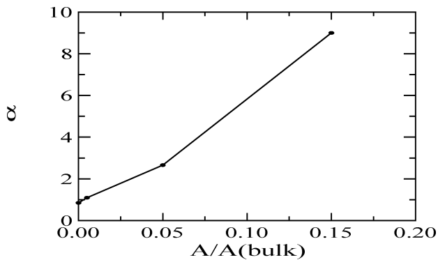
Fig. 6. Slope of the hysteresis loop as a function of the intergranular exchange coupling.
