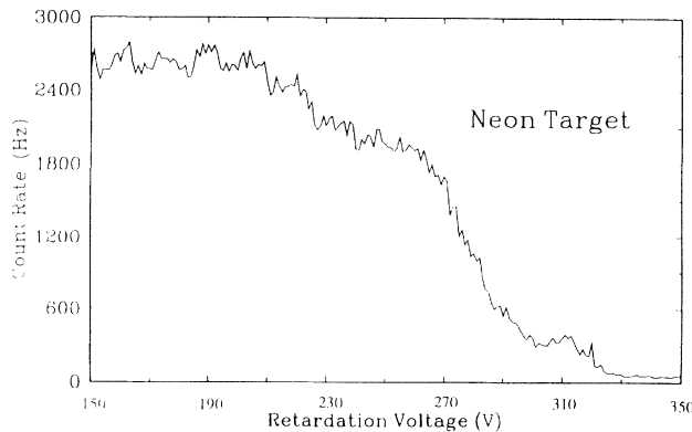
FIG. 8. Retarding-voltage spectrum of {}^3\text{He}^+ formed through the collision of 30-keV/u {}^3\text{He}^{2+} incident on neon.
