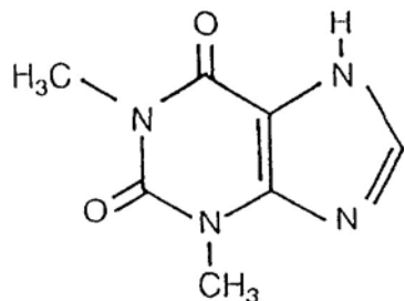
Figure 2. Structure of theophylline.
