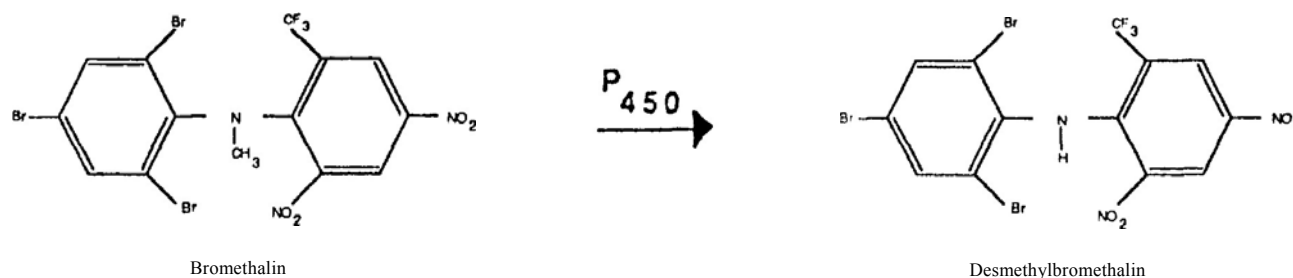
Figure 1. Metabolism of bromethalin.
