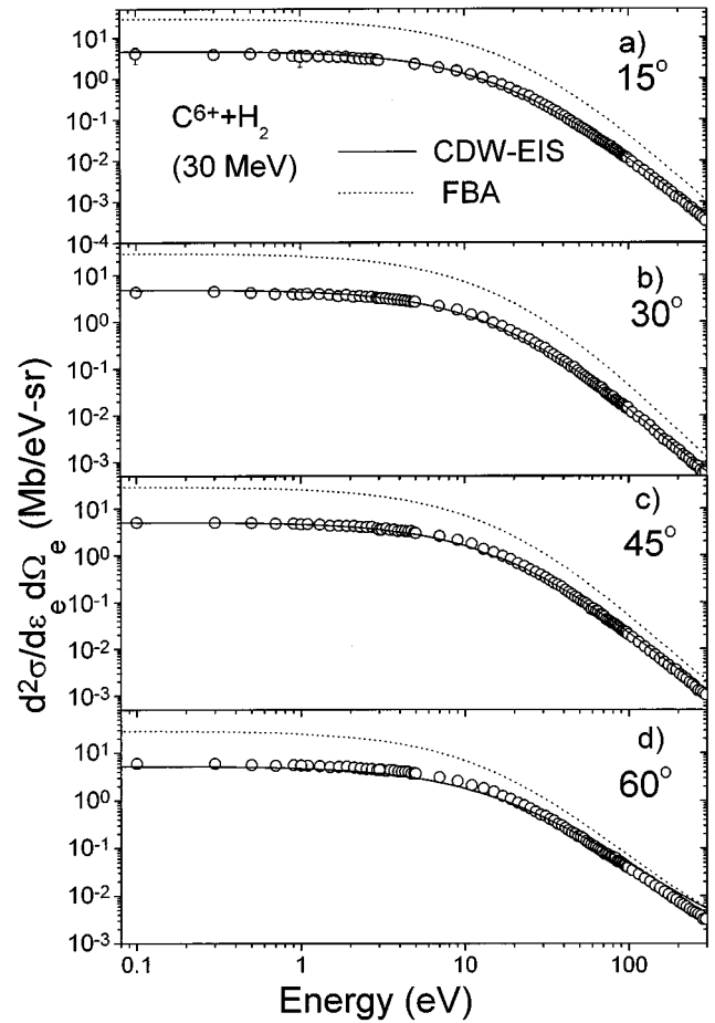
FIG. 1. (a) Double differential cross sections of electron emission for four different angles, namely, \theta_e = 15^\circ, 30^\circ, 45^\circ, and 60^\circ . The CDW-EIS and FBA calculations are shown by solid and dotted lines, respectively.
