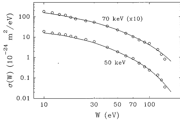
FIG. 3. Noncoincidence electron spectra from 50- and 70-keV \text{H}^- + \text{Ar} collisions. Solid lines, SDCS data from Rudd, Toburen, and Stolterfoht [14]; circles, relative SDCS data from this measurement normalized at 50 eV.
