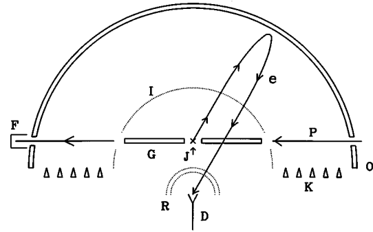
FIG. 2. Schematic diagram of the low-pass high-pass electron energy analyzer. P , projectile beam; G , beam guide; F , Faraday cup; J , Gas jet; e , typical electron trajectory; I , hemispherical grid; O , outer hemispherical electrode; K , guard rings; R , high-pass filter; D , electron detector.
