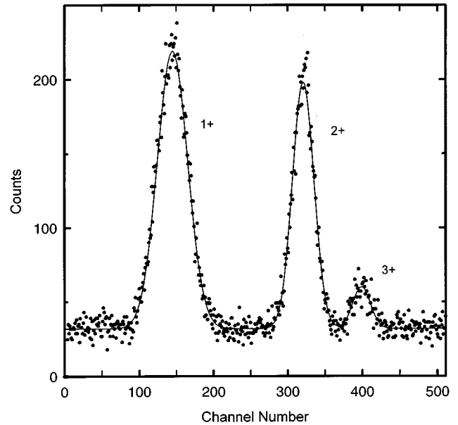
FIG. 4. Example of TOF coincidence spectrum for 50 eV electrons from 120-keV \text{H}^+ + \text{Ar} collisions.
