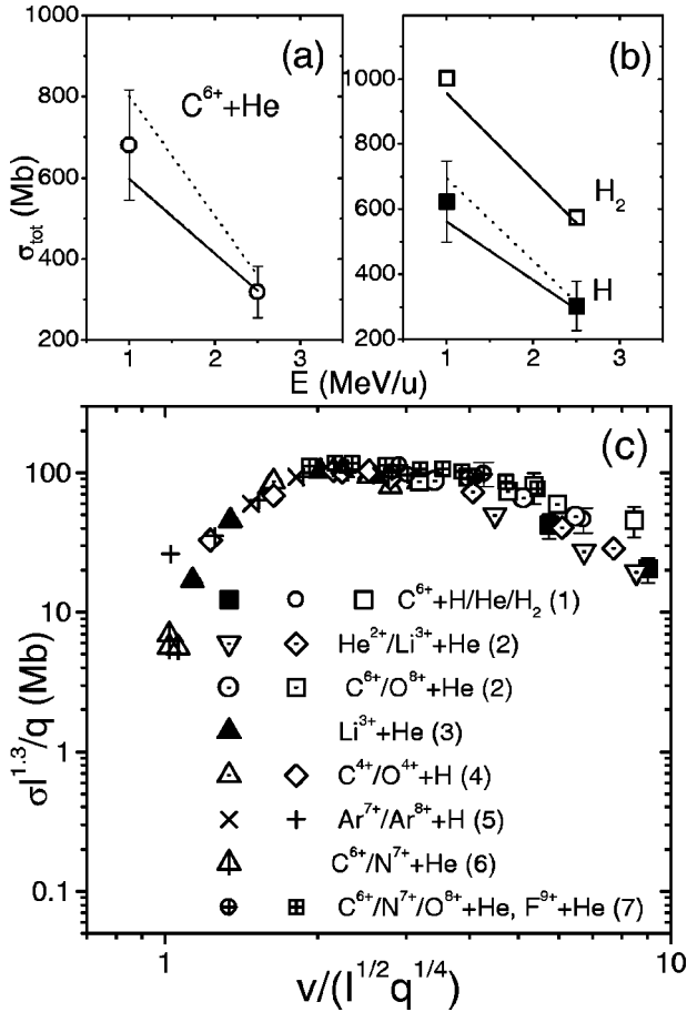
FIG. 7. The total ionization cross sections for \text{C}^{6+} + \text{He} (a) and \text{C}^{6+} + \text{H}_2 and \text{C}^{6+} + \text{H} (b) (paper I and Refs. [22,3]) at two collision energies. The scaled cross section vs the scaled velocity. The different sets of data are taken from the following references: (1) present and [22,3], (2) [27], (3) [26], (4) [25], (5) [24], (6) [18], and (7) [21].
