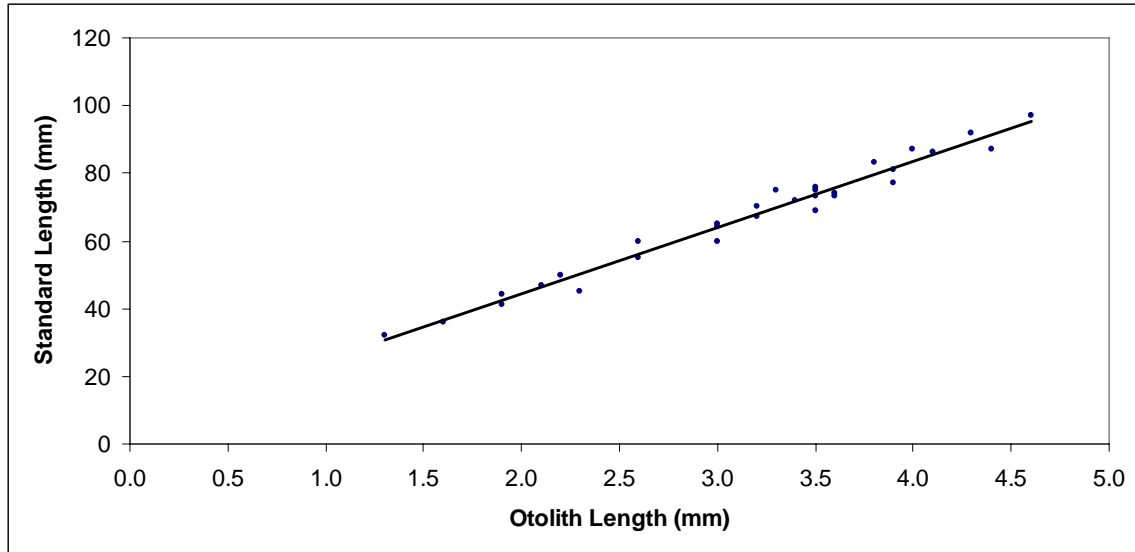
Figure 1. Linear regression of standard length on otolith length for Myctophum aurolaternatum .
