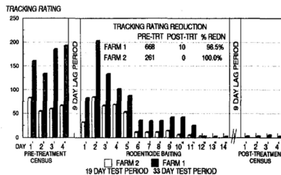
Figure 2b. Daily tracking ratings. UK field trials of 50 ppm brodifacoum blocks with Bitrex versus warfarin-resistant Norway rats.
