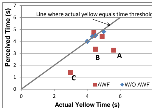
Fig. 8 – Comparison between actual and perceived yellow lengths
