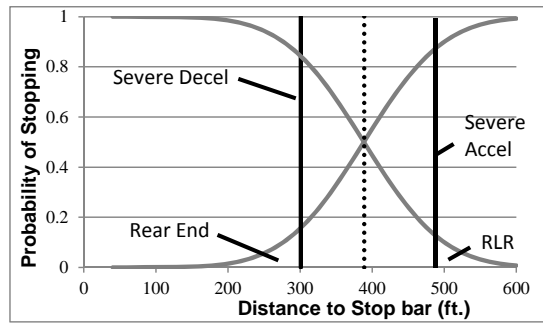
Fig. 1 - Critical distances along probability of stopping curve
