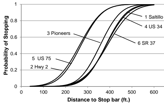
Fig. 3 - Critical distances along probability of stopping curve
