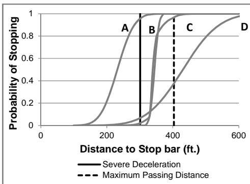
Fig. 7 – Hypothetical probability of stopping curves
