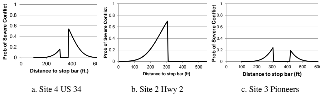
Fig. 4 - Probability of perceived traffic conflict at different sites
