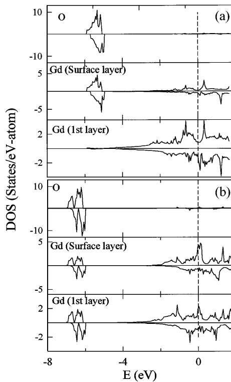
FIG. 3. The calculated partial density of states, reference to the Fermi level, of oxygen (top panel), the gadolinium surface (middle panel), and the first subsurface gadolinium layer (bottom panel) for (a) oxygen sites above the three fold hollow of the Gd surface and (b) for oxygen sites in the threefold hollow between the Gd surface layer and the next layer below.
