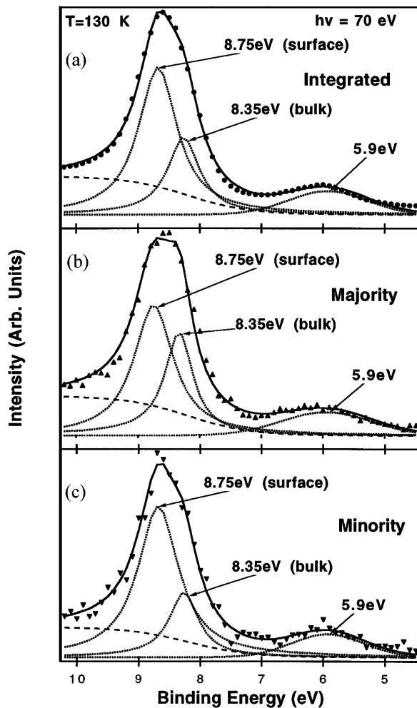
FIG. 1. Photoemission spectra of the 4f core levels of clean Gd(0001), (a) spin integrated, (b) the spin-majority component of the spin-integrated spectrum in panel (a) and (c) the spin-minority component of the spin-integrated spectrum in panel (a). The symbols are the data, and the solid lines are the fits of the data using a Doniach-Sinjac line shape. The dashed lines represent the deconvoluted surface and bulk components of the respective spectra. Panels (b) and (c) are expanded relative to (a) in order to show the details of the fits.
