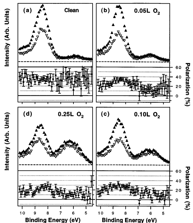
FIG. 2. The normalized spin-polarized photoemission spectra of the Gd 4f core levels as a function of oxygen exposure: (a) clean, (b) 0.05 L, (c) 0.10 L, and (d) 0.25 L. The closed triangles are the majority components, and the open triangles are the minority components. The polarization is displayed below each spectra.
