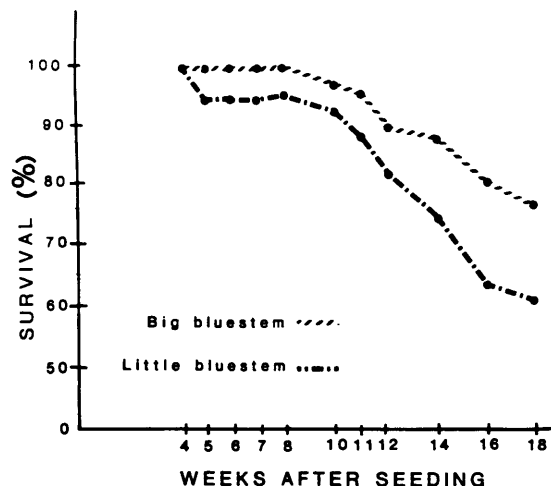
FIG. 2. Survival (%) for big and little bluestem averaged over the medium and high seeding rates at Harlan County, Nebraska. Percent survival was based on emerged seedlings following an 24 April 1982, sod seeding.
