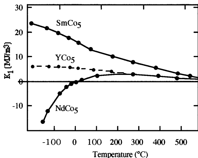
Fig. 2. Temperature dependence of the anisotropy of some \text{RCo}_5 intermetallics.
