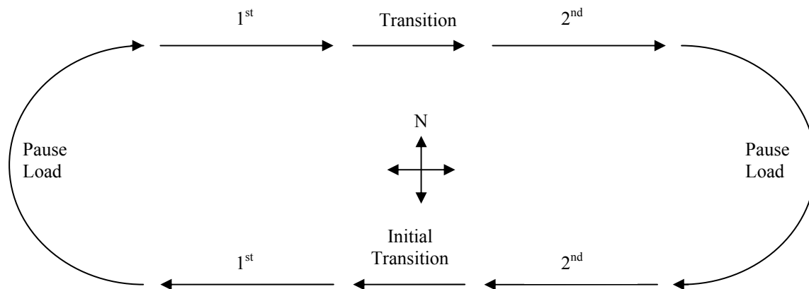
Figure 2. Test pattern used (trend continues for 3 rd through 6 th loads in randomized sequence of each block).
