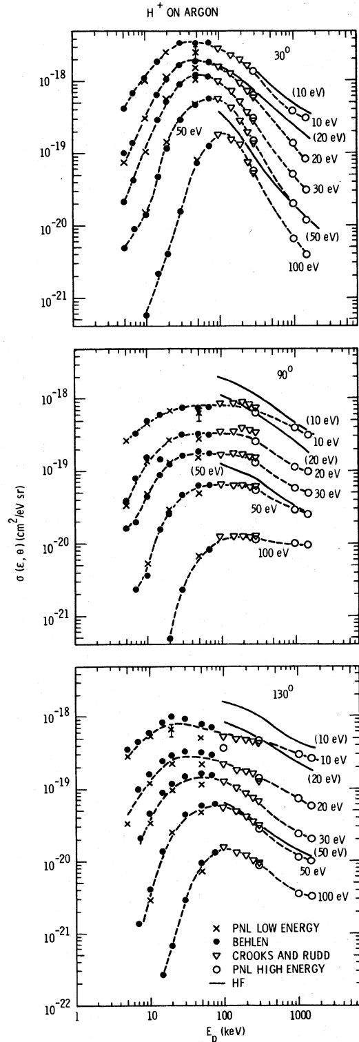
FIG. 9. Double-differential cross sections as a function of proton energy E_p : PNL low-energy apparatus ( \times ), Behlen ( \bullet ), Crooks and Rudd (Ref. 5) ( \nabla ), PNL high-energy apparatus ( \circ ), and the PWBA calculation of Manson (Ref. 4) (solid lines).
