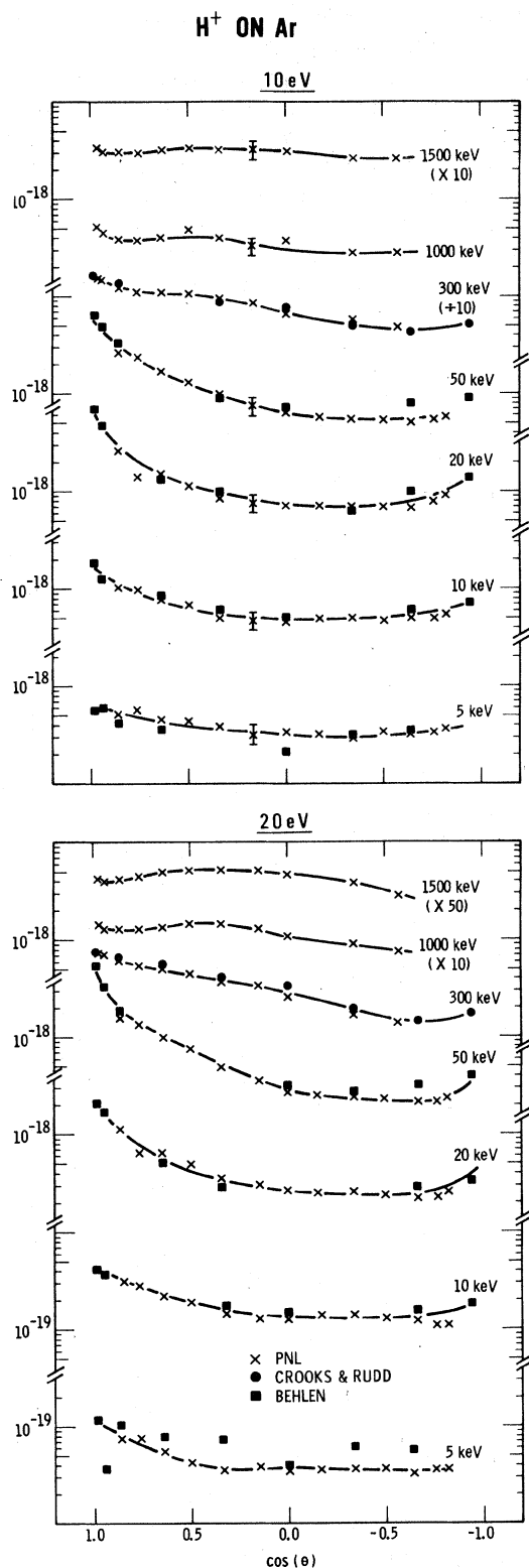
FIG. 4. Angular distributions of the double-differential cross sections for 10- and 20-eV electrons: PNL (x), Behlen (■), and Crooks and Rudd (Ref. 5) (●).
