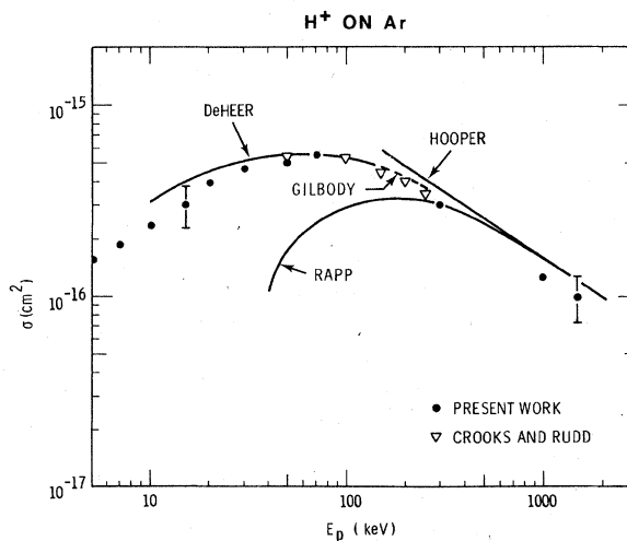
FIG. 6. Total ionization of argon by protons and electrons. Protons: ●, present work; ▽, Crooks and Rudd (Ref. 5), De Heer et al. (Ref. 17), Gilbody and Lee (Ref. 15), Hooper et al. (Ref. 14). Electrons: Rapp and Englander-Golden (Ref. 16).
