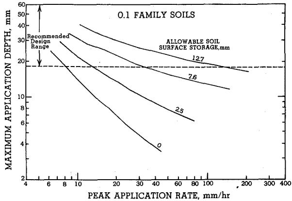
FIG. 4.—Maximum Depth of Water Application per Irrigation for 0.1 Family Soil
