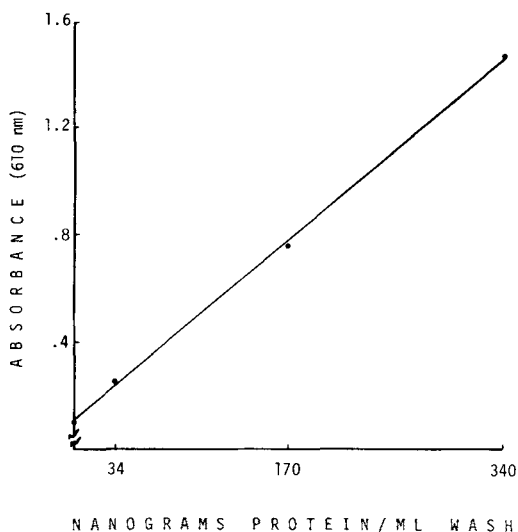
FIG. 1. Standard curve to relate protein in a test-wash solution to absorbance of the destain solution.
