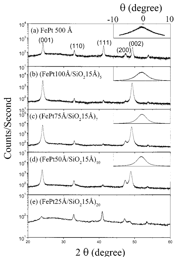
FIG. 1. XRD scans of (FePt x Å/SiO 2 15 Å) n multilayers annealed at 650 °C for 2 h. The insets are the (001) peak rocking curves.
