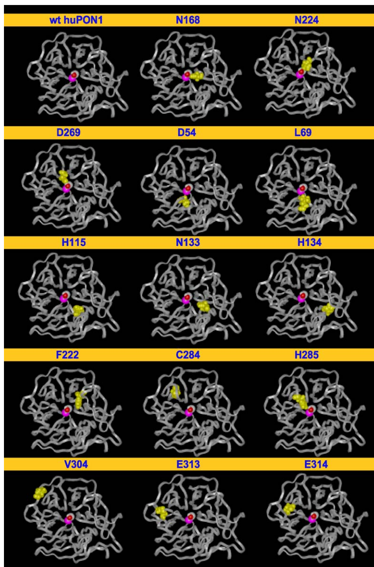
Fig. 3. Graphical depictions of residues selected for mutation (in yellow, as space-filling representations) and their relative locations in the ribbon backbone of the proposed HuPON1 structure are shown. The theoretical catalytic calcium is shown in white along with a modeled water molecule (red and gray), and the proposed structural calcium is shown in pink.
