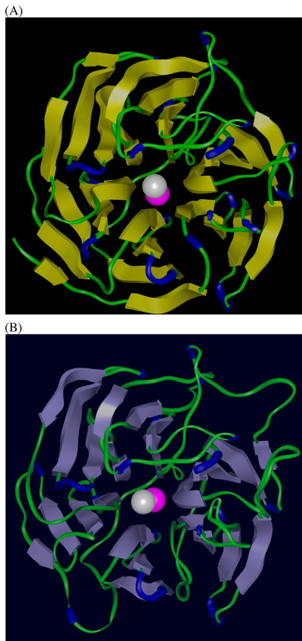
Fig. 1. (A) View of a ribbon diagram of the DFPase structure as determined from X-ray crystallography experiments [23]. (B) Ribbon diagram representation of the proposed secondary structure of HuPON1 viewed along the axis with the catalytic calcium (white) above the structural calcium (pink). The model displays a slightly distorted six-bladed \beta -propeller shown in the same relative orientation as (A). HuPON1 was simulated using explicitly solvated dynamics with Insight/Discover software from Accelrys. Computational resources were provided by the National Cancer Institute's Advanced Biomedical Computing Center in Frederick, Maryland.
