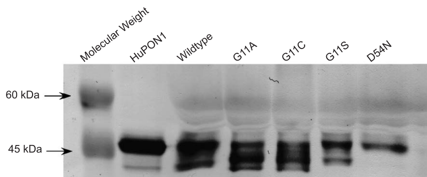
Fig. 4. Western blot of purified native HuPON1, recombinant wild-type and selected mutants. Each lane was loaded with 40 μl of recombinant HuPON1 in culture medium and SDS Laemmli sample buffer (1:1 v/v). Samples were transferred to PVDF membrane and probed with a monoclonal mouse anti-HuPON1 antibody and probed with alkaline-phosphatase conjugated rabbit anti-mouse antibody. Images were developed via BCIP/NBT liquid substrate system and visualized by scanning. Comparable blots were obtained with mutants L69F, H115W, N133S, H134W, H134Y, N168E, F222D, F222Y, N224A, D269E, C284D, H285D, H285Y, V304A, E313A, E314A, and the double mutant H115W/N133S (data not shown).
