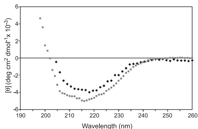
Fig. 2. CD spectra of HuPON1 purified from serum in the presence of either TX-100 or BOG at 25 °C. The spectra of HuPON1 were plotted to exclude low wavelength data prone to error due to light scattering of the TX-100 or BOG detergents. The data were plotted over a range of wavelengths that gave an error of less than 25%. Gray squares: from 198–260 nm, 3.0 µM HuPON1 in 0.1% BOG, or Black diamonds: from 205–260 nm, 0.64 µM HuPON1 in 0.01% TX-100. The mean residue ellipticity reported has been corrected for molar protein concentration, path length and amino acid residue in HuPON1 as described in Materials and methods.
