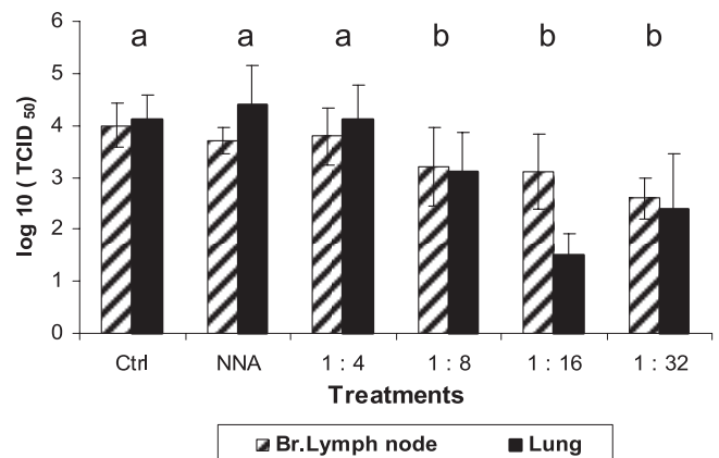
FIG. 2. Correlation between the titer of NA and the viral load in bronchial lymph nodes and lungs. Fifteen-day-old pigs were passively transferred with either neutralizing immunoglobulins to attain titers of 1:4, 1:8, 1:16, and 1:32, non-neutralizing antibodies (NNA), or no antibodies (Ctrl) and challenged with PRRSV 1 day later (experiment 1). The virus titers in the bronchial lymph nodes (▨) and lungs (■) at day 7 p.i. are shown. Columns with different letters are marginally significantly different in the lymph nodes ( P = 0.06 ) and significantly different in the lung ( P < 0.05 by Student t test, 11 df). Ctrl, animals were not transferred with antibodies; NNA, animals were transferred with non-NA. Groups 1:4, 1:8, 1:16, and 1:32 indicate the different groups of animals that, when passively transferred with different quantities of NA, attained peripheral SVN titers of 1:4, 1:8, 1:16, and 1:32, respectively.
