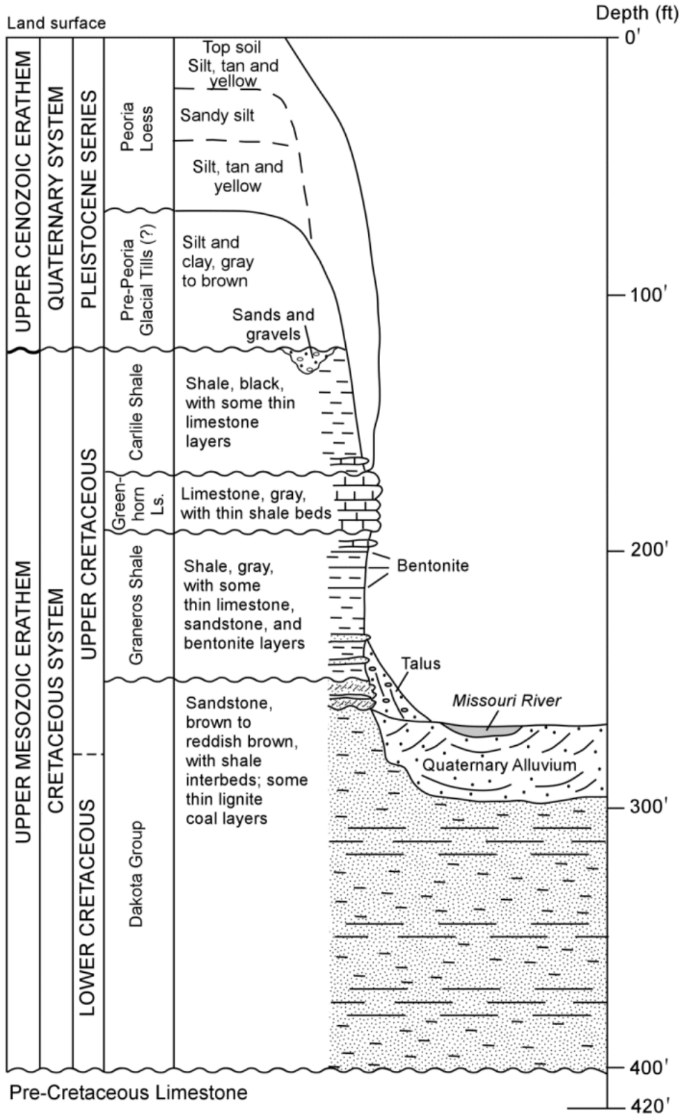
General Geologic Section From Ponca State Park Resource and Education Center To The Missouri River Boat Ramp
