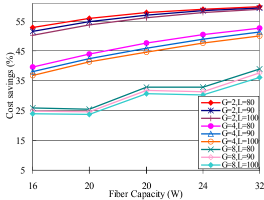
Fig. 20. Cost savings of the IIWBS algorithm on the NSF network under different fiber capacities, where \alpha = 5 and \beta = 1 .
