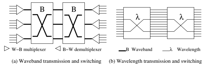
Fig. 1. Comparison of waveband switching and wavelength switching along a two-hop route.
