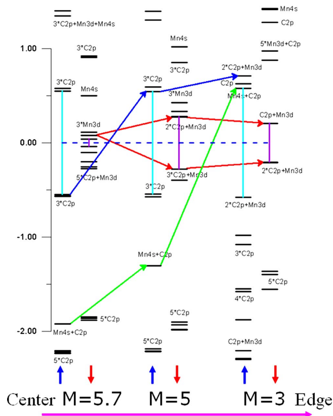
FIG. 6. (Color online) Molecular orbital energy diagrams for \alpha and \beta spin electrons with different spins obtained using scheme 1. Zero energy is chosen to be the center of each HOMO-LUMO gap.
