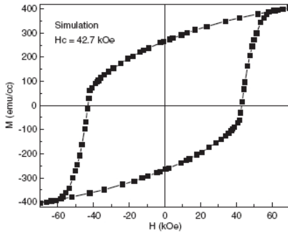
Fig. 11. Simulated hysteresis for assembly of isolated nanoclusters.
