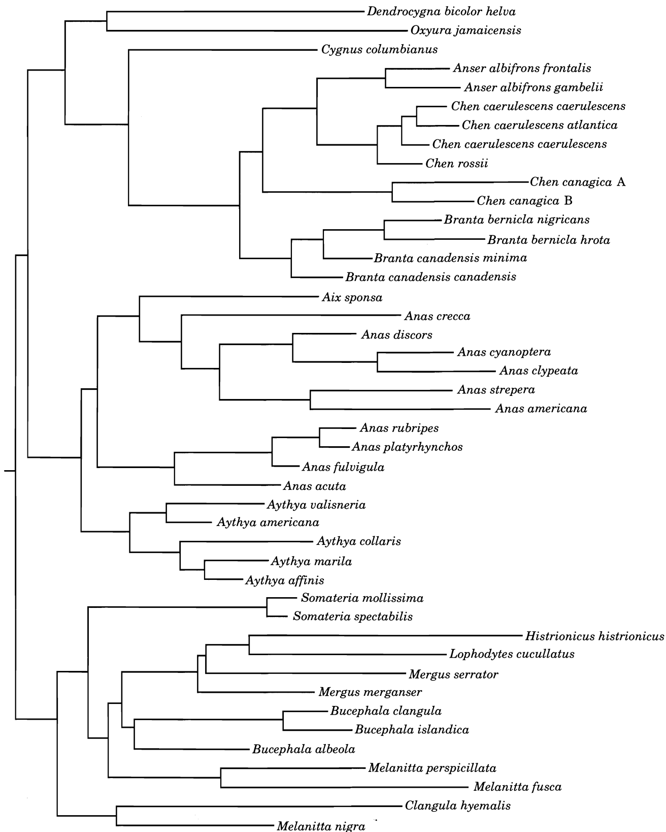
Figure 2. Distance Wagner Diagram for the family Anatidae constructed using modified Rogers' distance measure ( D_r ) and distance Wagner procedure of Swofford (1981).
