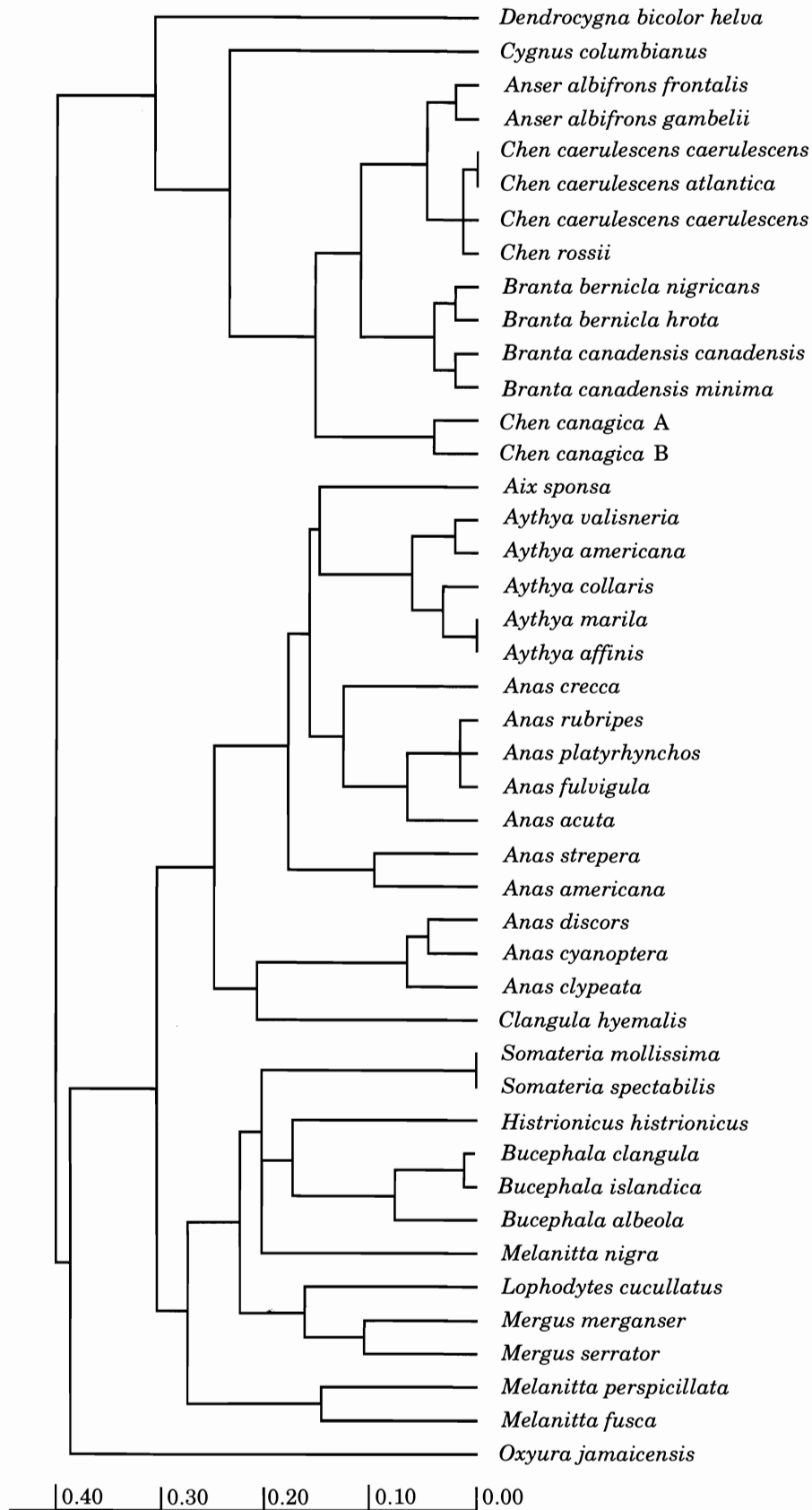
Figure 1. Phenogram constructed using the unweighted pair-group method with arithmetic averages (UPGMA) from a matrix of D-values. Phenetic relationships of the family Anatidae based upon Nel's (D) (Nel, 1978).
