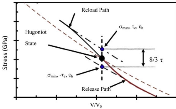
Fig. 5. Reshock/release experimental results used to depict technique to estimate the shear stress state, \tau_h , and the maximum strength, \tau_c , the material can sustain at a Hugoniot strain of \epsilon_h . This allows us to determine the mean stress state, P , for the materials.
