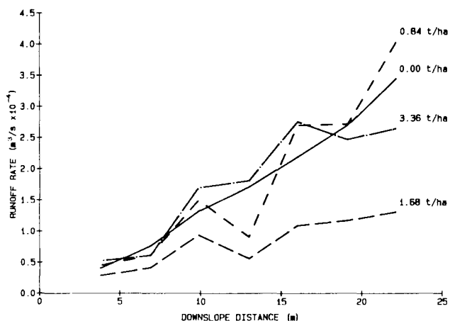
Fig. 2a—Runoff rate in rills or overland flow channels at selected downslope distances for four soybean residue treatments.
