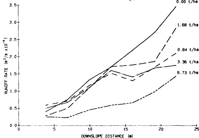
Fig. 1a—Runoff rate in rills or overland flow channels at selected downslope distances for five sorghum residue treatments.
