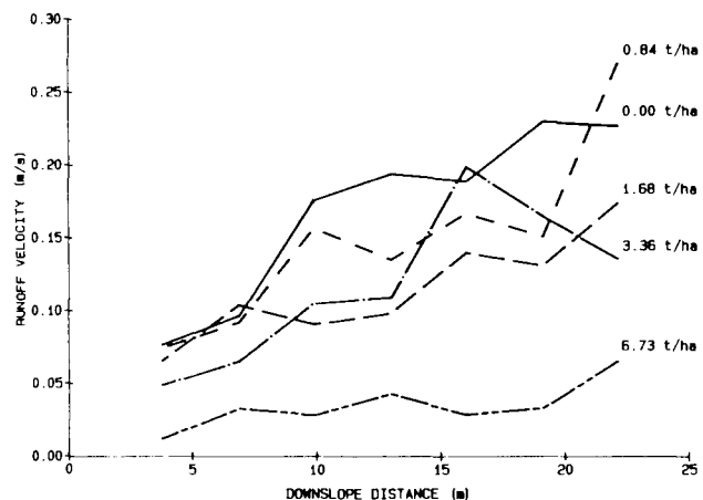
Fig. 2b—Runoff velocity in rills or overland flow channels at selected downslope distances for five soybean residue treatments.
