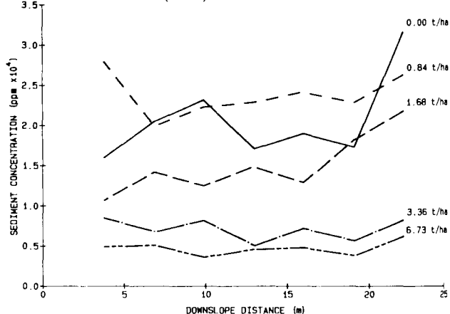
Fig. 1c—Sediment concentration in rills or overland flow channels at selected downslope distances for five sorghum residue treatments.
