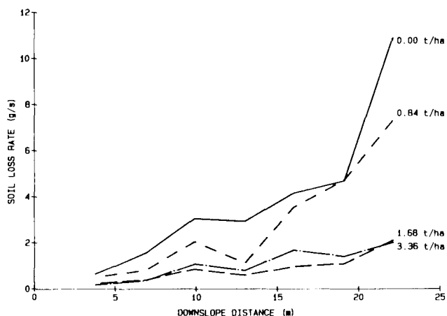
Fig. 2d—Soil loss rate in rills or overland flow channels at selected downslope distances for four soybean residue treatments.
