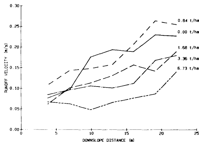
Fig. 1b—Runoff velocity in rills or overland flow channels at selected downslope distances for five sorghum residue treatments.
