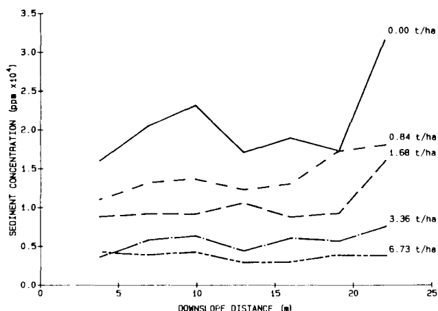
Fig. 2c—Sediment concentration in rills or overland flow channels at selected downslope distances for five soybean residue treatments.
