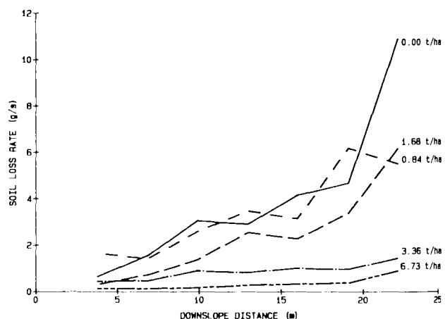
Fig. 1d—Soil loss rate in rills or overland flow channels at selected downslope distances for five sorghum residue treatments.
