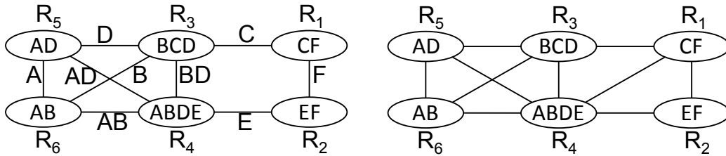
Figure 13: Triangulating a dual graph.
