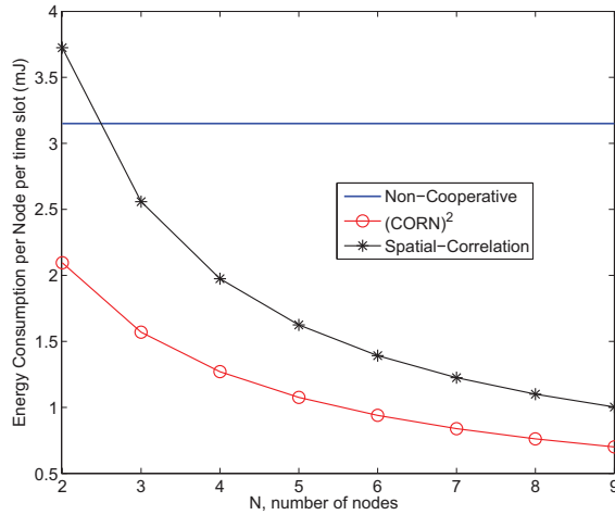
Fig. 4. Energy consumption vs. number of nodes N . R_D = 0.9 , R_S = 0 , w_{ij}(t) = 0.6 .
