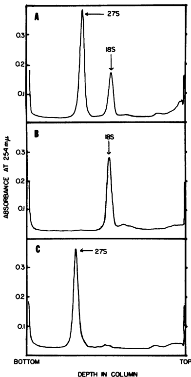
FIG. 2. Sedimentation pattern of ribosomal RNA from spore ribosomes and ribosomal subunits. Centrifuged on sucrose "linear log" gradient columns (3) equilibrated with 0.15 \text{ M NaCl} and 0.015 \text{ M} sodium citrate ( \text{pH } 7.0 ). Brome mosaic virus and tobacco mosaic virus RNA species were used as markers for determining the sedimentation constants of the ribosomal RNA species. The ribosomal RNA was analyzed after stripping the ribosomes of protein by incubation in 0.01
