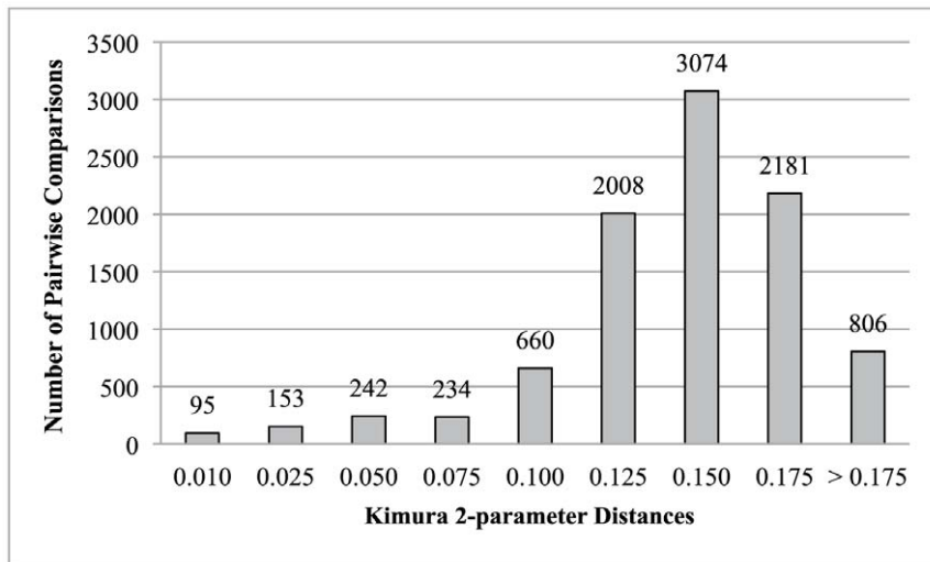
Figure 3. Kimura 2-parameter pairwise distances based on cytochrome- b sequence data. Y-axis indicates the number of total pairwise comparisons of sequences and the X-axis indicates the Kimura 2-parameter distance values among ingroup taxa. Note the large portion of pairwise values over 10% (average divergence of 13.14%). doi:10.1371/journal.pone.0046578.g003
