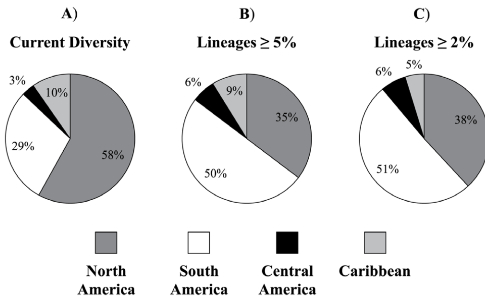
Figure 4. Diversity estimates based on currently recognized species and genetic lineages presented herein. The number of lineages restricted to each region (distributions based on [12–16]) is shown as a percentage of the total. A) percentage of diversity in each region based on currently recognized diversity, B) percentage of diversity in each region based on a species divergence level set at \geq 5.0\% using cytochrome- b DNA sequence data, C) percentage of diversity in each region based on a species divergence level set at \geq 2.0\% . Note the proportion of lineages from each region changes from the current levels, when compared to the lineages at 5.0% and 2.0%. doi:10.1371/journal.pone.0046578.g004
