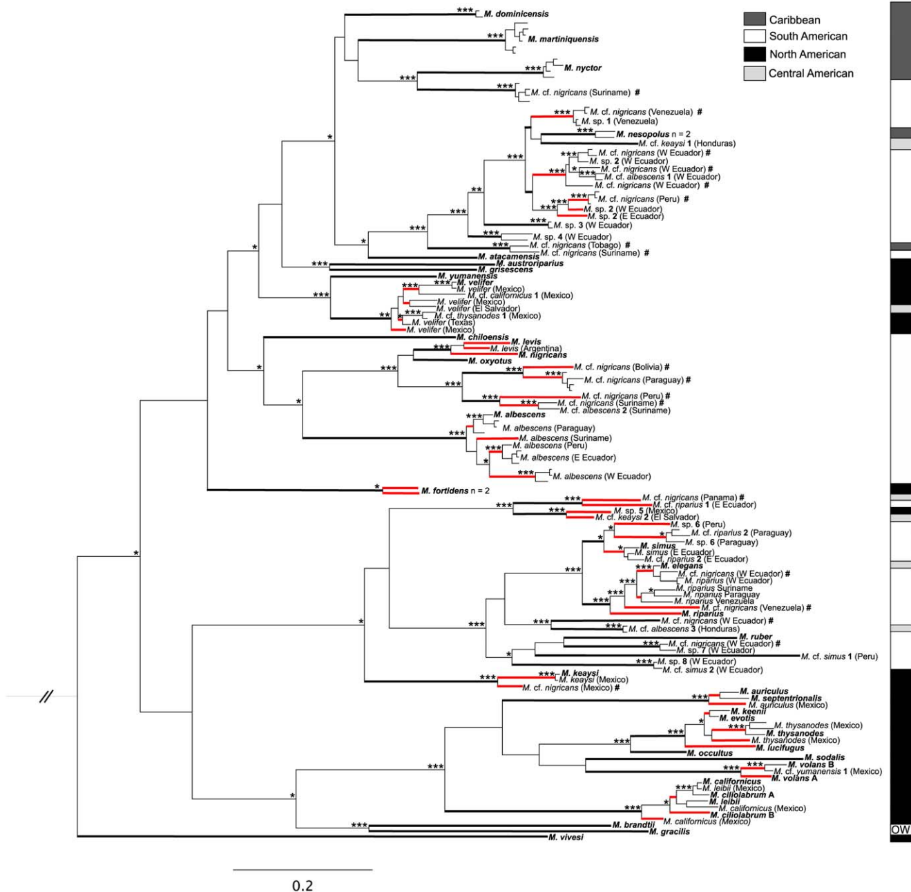
Figure 2. Bayesian phylogram of cytochrome- b sequence data (n = 140). Species names are based on museum and field records. Bolded species names are currently recognized by Simmons [13] and serve as the species representative (from GenBank [2,3,16] or from specimens sequenced herein). Black bolded branches are lineages that are \geq 5.0\% divergent and red bolded branches are lineages \geq 2.0\% divergent. Bolded numbers within species names indicate specimens that were originally identified as the named species, but were found to be independent lineages that are \geq 5.0\% divergent. The pound sign (#) indicates all specimens originally identified as M. nigricans . OW = Old World lineages of M. brandtii and M. gracilis . Kerivoula papillosa and M. latirostris are outgroup taxa but are not shown in the phylogram. Support for nodes are presented as Bayesian posterior probabilities \geq 0.95 (*), maximum likelihood bootstrap pseudo-replicate values \geq 75\% (**), or support in both analyses (***). Additional specimen information is in Table S1. doi:10.1371/journal.pone.0046578.g002
