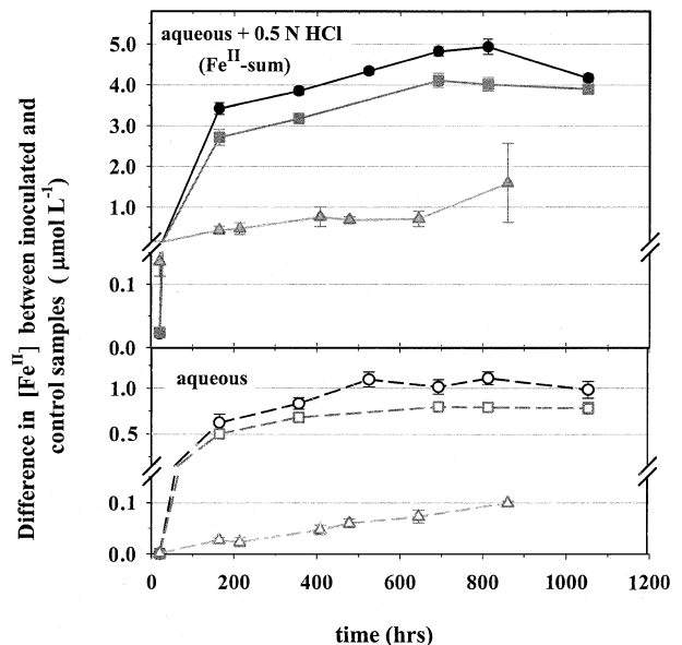
Fig. 3. \text{Fe}^{\text{II}} generation as a function of time during sediment reduction by S. putrefaciens . Note the split axes. Open symbols represent \text{Fe}^{\text{II}} -aq (bottom), solid symbols represent sum of aqueous and 0.5 N HCl-soluble, surface-bound \text{Fe}^{\text{II}} (top). Circles = VHSA-G. squares = Fe-K-Q. triangles = H-sand. Data are normalized by subtracting values from uninoculated controls, and error bars represent the standard deviation of three replicate samples.
