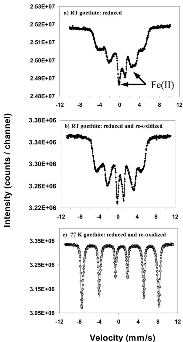
Fig. 4. Room temperature (RT) and 77 K Mössbauer spectra of microbially reduced VHSA-G and microbially reduced VHSA-G that has been reoxidized. All samples are in the presence of 225 \mu\text{M Zn}^{\text{II}} . (a) RT reduced, (b) RT reduced and reoxidized, (c) 77 K reduced and reoxidized. Marked peaks indicate regions of the RT spectra that are enhanced by \text{Fe}^{\text{II}} generation. (a, b) Points and line represent the same data set. (c) Points represent data and line equals model fit for goethite.
