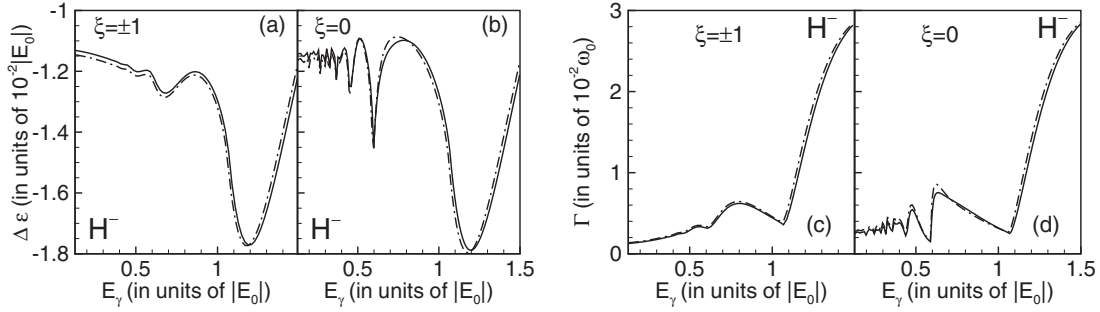
FIG. 3. Variation of the complex quasienergy of H^- with photon energy E_\gamma = \hbar\omega for a laser field of intensity I = 1.84 \times 10^{11} W/cm 2 and for both circular ( \xi = \pm 1 ) and linear ( \xi = 0 ) polarizations. Solid lines: TDER results. Dot-dashed lines: RZRP results ( r_0 = 0 ). For \omega_0 , see Fig. 1(c).
