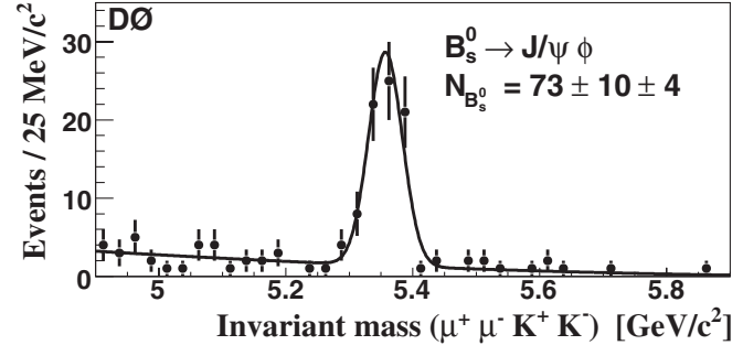
FIG. 2. The invariant mass distribution of the normalization channel B_s^0 \rightarrow J/\psi \phi after all selection criteria.
