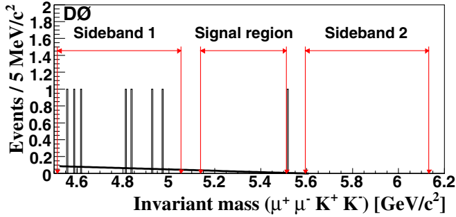
FIG. 1 (color online). The invariant mass distribution after optimized requirements on the discriminating variables. The solid line shows the sidebands background interpolation into the signal region.
