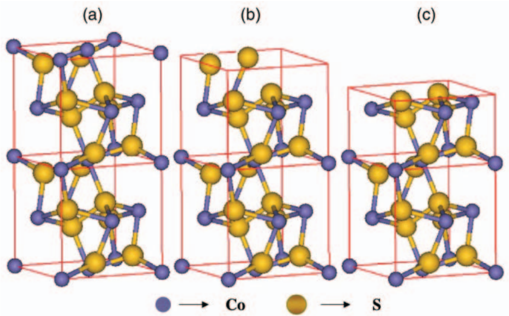
Figure 3. Schematic diagram of possible terminations of the \text{CoS}_2(100) surfaces: (a) Co-terminated, (b) 2S-terminated (by removing a Co layer from the Co-terminated structure) and (c) 1S-terminated (by removing the surface S layer from the 2S-terminated structure). See reference [12].
