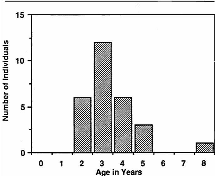
FIGURE 7. Age distribution of Natural Trap Cave bighorn sheep. Derived from cemental annulation of left incisors (see text). Sample size of incisors: 28.
