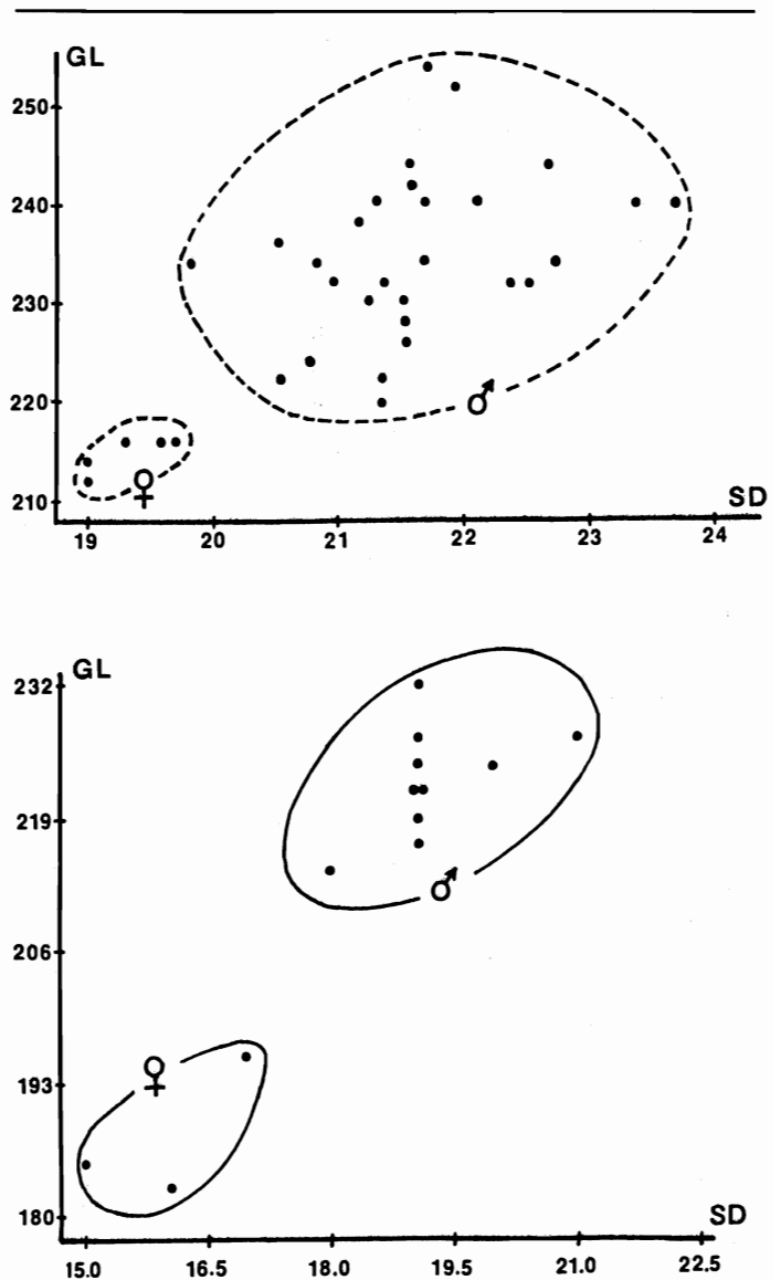
FIGURE 8. Plots of measurements of greatest length (GL) over smallest breadth (SD) of metatarsals, showing sexual dimorphism. Upper: Natural Trap Cave sheep. Lower: modern O. c. canadensis (measurements of University of Montana sample).
