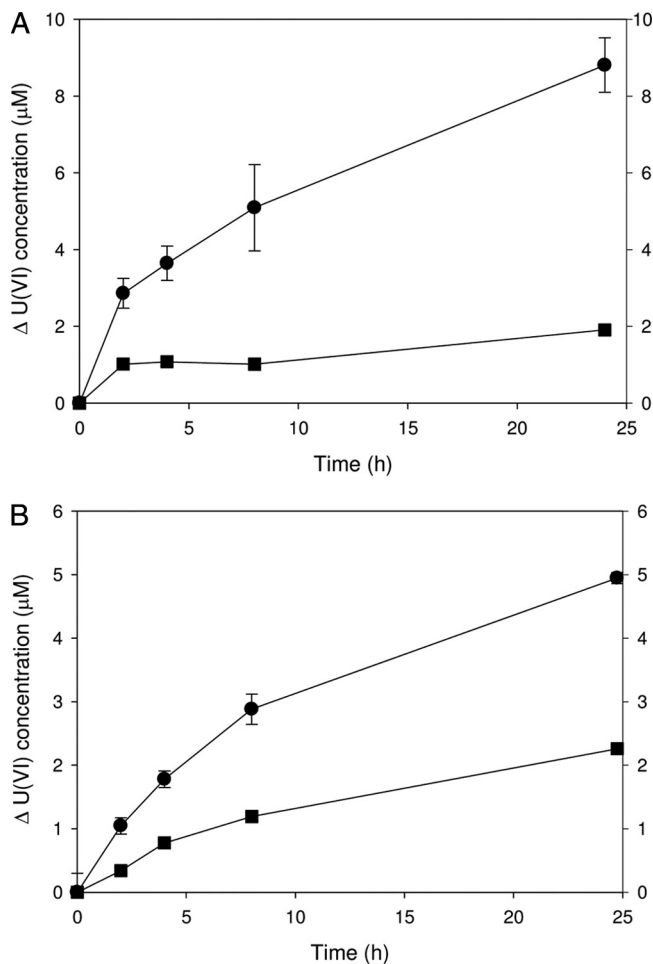
FIG. 1. Nongrowth cell suspension experiments were conducted in 30 mM bicarbonate buffer (pH 6.8, N 2 -CO 2 headspace) containing chemically precipitated UO 2 and nitrate inoculated with a live, washed cell suspension of A. ebreus strain TPSY (A) and Pseudogulbenkiania sp. strain 2002 (B) grown on acetate and nitrate (6.25 mM and 10 mM, respectively) with results compared to those of pasteurized control cultures. ●, live cells; ■, pasteurized cells. Symbols represent average results for triplicate cultures. Error bars denote standard error of measure.
