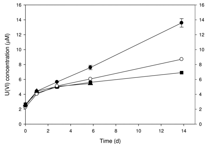
FIG. 2. Anaerobic, nitrate-dependent U(IV) oxidation by Pseudogulbenkiania sp. strain 2002 under growth conditions in basal bicarbonate buffer (pH 6.8, N 2 -CO 2 headspace) containing chemically precipitated UO 2 and nitrate. ●, live cells; ■, pasteurized cells; ○, live cells amended with sodium azide (electron transport inhibitor); ▲, live cells with U(IV) only (no nitrate). Symbols represent average results for triplicate cultures. Error bars denote standard error of measure.
