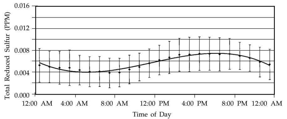
Figure 2. Average TRS concentration (reported as an H 2 S equivalent) vs. time of day for feedlot #3 during Spring 2001.
