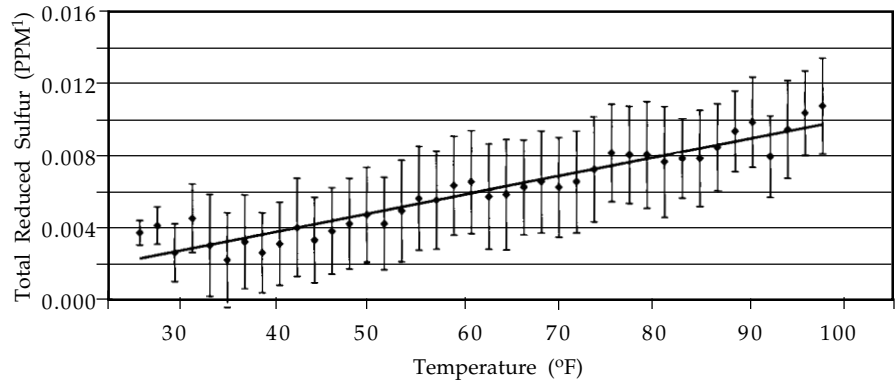
Figure 1. Average TRS concentration (± one standard deviation) vs. Air Temperature for Feedlot #3 during Spring 2001.
