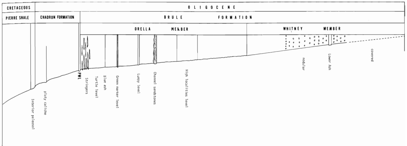
FIGURE 2.—Generalized stratigraphic section, Chadron area, eastern Dawes County, Nebraska. This section was developed from a series of isolated exposures north of and west of Chadron, and does not include the Pine Ridge escarpment
