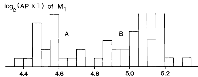
FIGURE 5.—Histogram of \log_e (AP, anteroposterior length \times T, transverse width) for lower first molars (no more than one measurement per individual was used) for all measurable oreodont specimens from the Dead Horse Local Fauna. Specimens falling below 4.75 were sorted into one group, those above 4.8 were sorted into a second group. Standard statistics for these groups are as follows:
