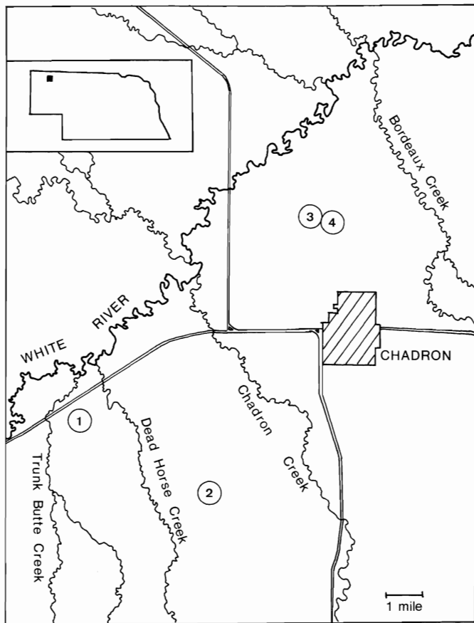
FIGURE 1.—Map of Chadron area, eastern Dawes County, Nebraska. Inset map shows general location. Circled numbers indicate locations of measured sections (Fig. 3).
