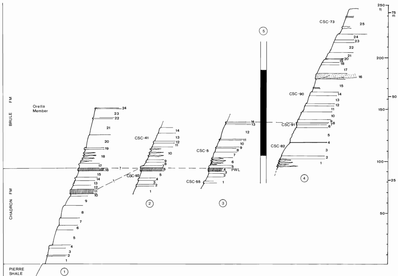
FIGURE 3.—Measured stratigraphic sections used in construction of the local standard section, Figure 4. Locations of these sections are indicated on Figure 1. Stratigraphic positions of Chadron State College localities are indicated on the section measured closest to the locality. Scale at right indicates distance above Pierre Shale only for Section 1; Sections 2-4 are tied by means of marker beds indicated.
