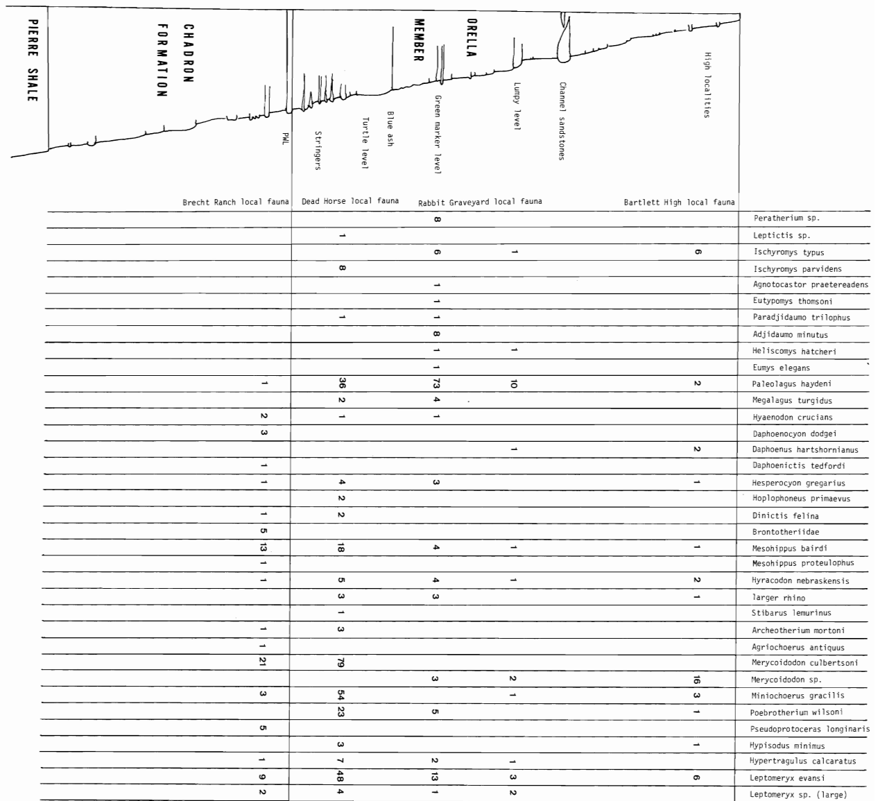
FIGURE 4.—Faunal checklist. Numbers indicate total number of recorded specimens (Chadron State College Collection) from a particular stratigraphic level. The Daphoenictis tedfordi specimen is F:AM 25,242, Frick Collection, American Museum of Natural History. Chadron State College localities used in local fauna specimen counts include:
