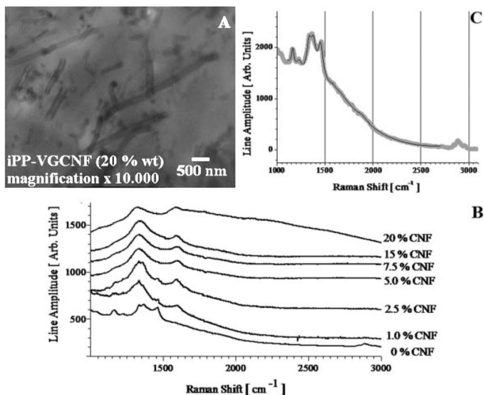
Figure 1. A: TEM photo of iPP-VGCNF composite; B: Raman spectra of iPP filled with various amounts of VGCNFs (expressed in wt %); and C: The best fit of Raman spectrum in the range 1000–2800 cm -1 for the pristine polymer.
