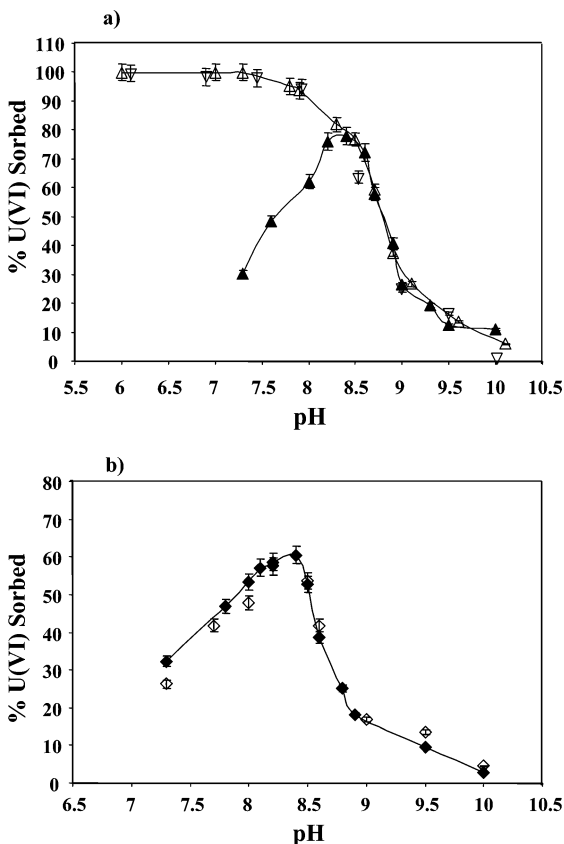
FIGURE 2. U(VI) sorption as a function of pH in five systems. (a) Three sorption systems with acid-washed solids: \blacktriangle = carbonate-free HSC silt/clay in calcite-presaturated solution; \triangle = carbonate-free HSC silt/clay in \text{Ca}^{2+} -free solution; \nabla = both carbonate- and iron-(hydr)oxide-free silt/clay in \text{Ca}^{2+} -free solution. (Initial [\text{U(VI)}] = 1.2 \times 10^{-6} mol/L, solid/solution ratio = 100 g/L, I = 0.05 mol/L ( \text{NaNO}_3 ), P_{\text{CO}_2} = 10^{-3.5} atm, and T = 22.5 °C.) Note that only the systems with open symbols are calcium-free. (b) Two sorption systems with untreated HSC silt/clay: \blacklozenge = untreated HSC silt/clay with calcite-presaturated solution; \diamond = untreated HSC silt/clay with initially \text{Ca}^{2+} -free solution. (Initial [\text{U(VI)}] = 1.2 \times 10^{-6} mol/L, solid/solution ratio = 100 g/L, I = 0.05 mol/L ( \text{NaNO}_3 ), P_{\text{CO}_2} = 10^{-3.5} atm, and T = 22.5 °C.) Note that neither system is calcium-free at equilibrium conditions.
