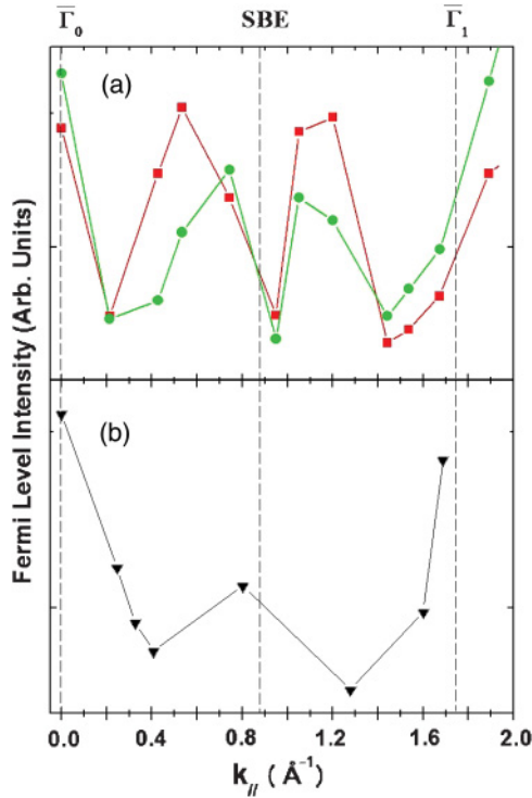
FIG. 6. (Color online) The Fermi-level intensity plotted as a function of the parallel momentum k_{\parallel} along the \overline{\Gamma M} direction, for photon energies of (a) 40 eV and (b) 25 eV. For k_{\parallel} along the \overline{\Gamma M} direction, the relative intensity has been also plotted 300–400 meV below the Fermi level (green ●) and at the Fermi level (red ■), to illustrate the roughly parabolic shape of the electron pocket about the surface Brillouin-zone edge at 40 eV.
