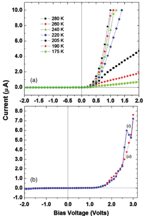
FIG. 9. (Color online) I - V curves for (a) undoped EuO(100) film as a function of temperature, (b) Eu 0.96 Gd 0.04 O(111) film at room temperature. The curve marked (i) is for zero field; the curve marked (ii) is for an external magnetic field of 1000 Oe.
