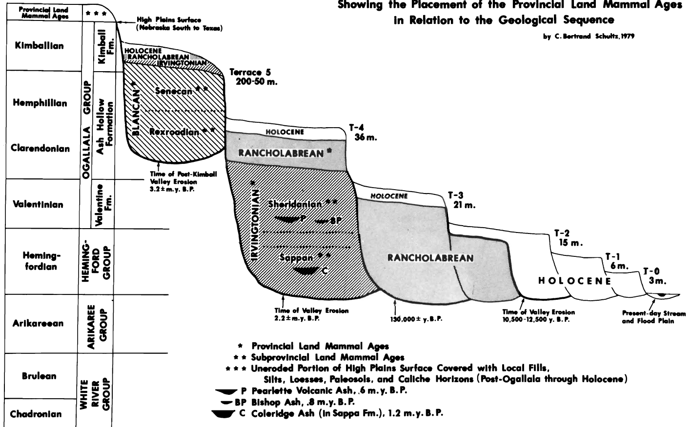
FIGURE 1. Diagrammatic or ideal cross-section of the main stratigraphic units of the Tertiary and Quaternary of the Great Plains of North America, showing the placement of the Provincial Land Mammal Ages in relation to the geological sequence. [Subdivisions of Quaternary Provincial Land Mammal Ages from Schultz, Martin, Tanner, and Corner (1977 and 1978); Figure from Schultz (1979 and 1981).]
