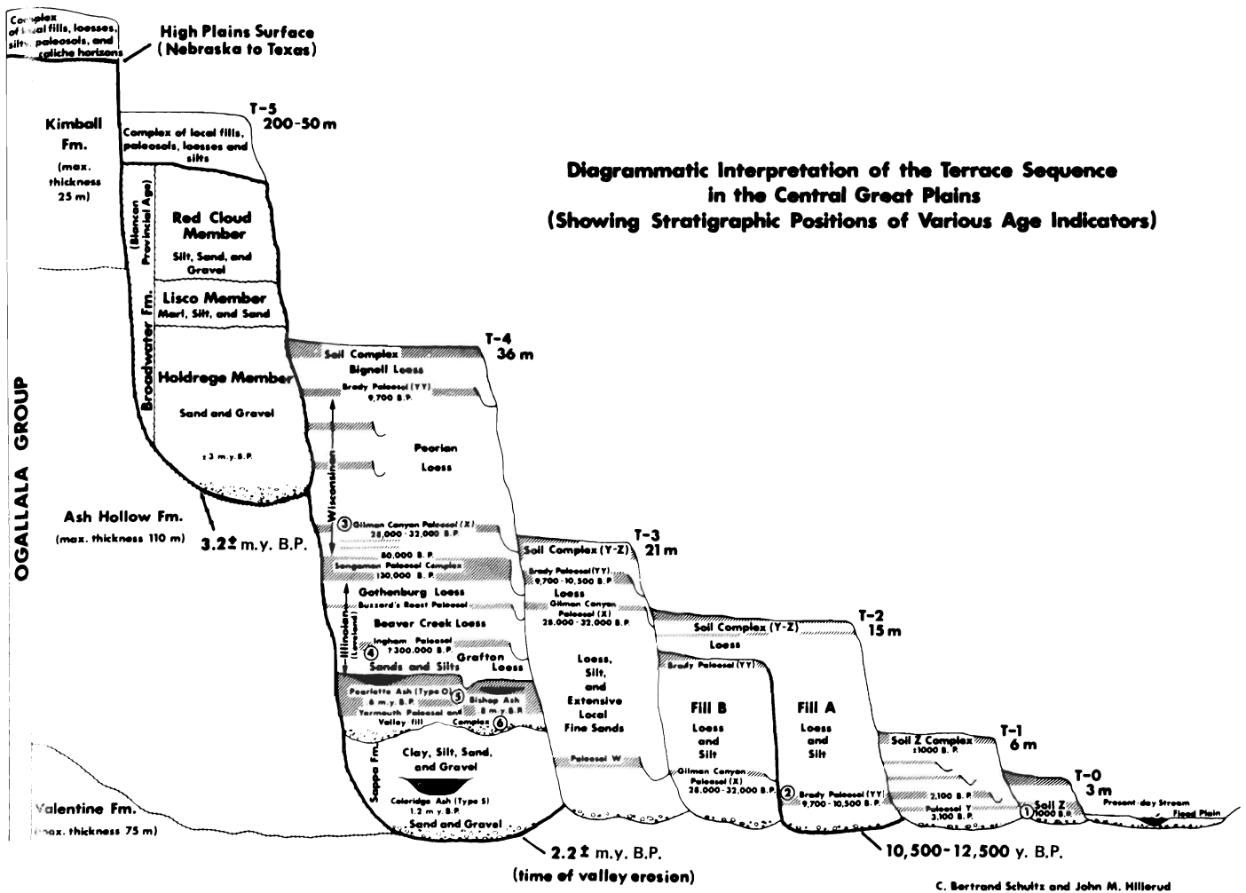
FIGURE 2. Diagrammatic interpretation of the terrace sequence in the Central Great Plains (showing stratigraphic positions of various age indicators). (From Schultz and Hillerud, 1978.)
