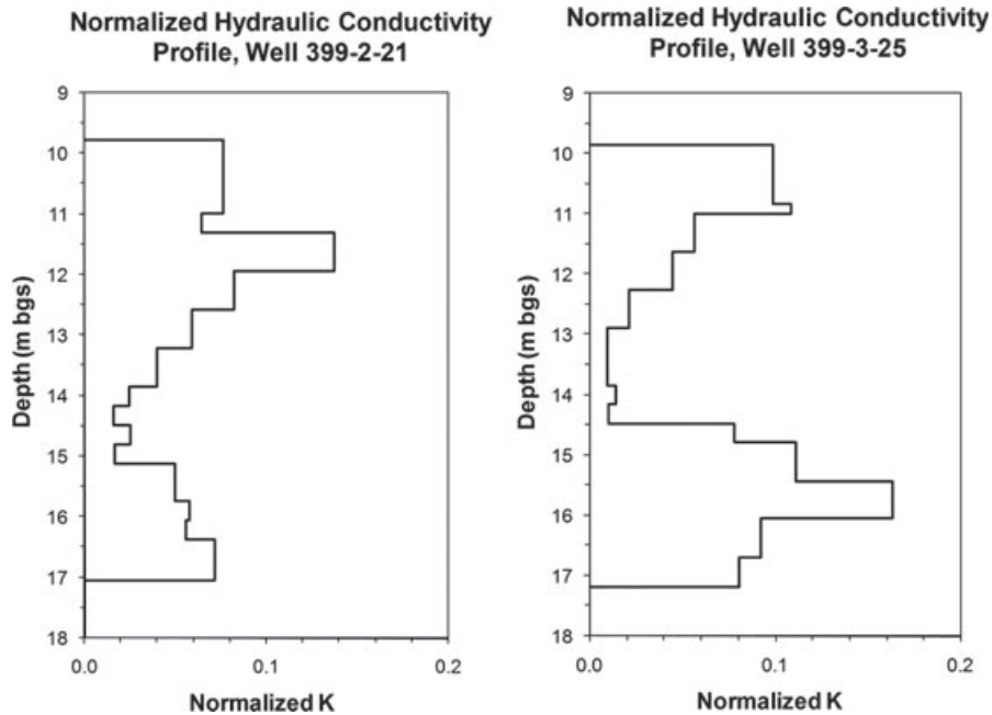
Figure 4. EBF profiles for the fully screened well used in this study (399-2-21) and adjacent well 399-3-25.
