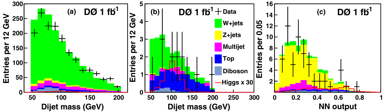
FIG. 1 (color online). The dijet mass distribution for all tau types for the \tau\nu analysis (a) before b tagging, and (b) after the final selection; (c) the combined NN_{Zjets} variable for the low Higgs boson mass \tau\tau analysis. The signal is shown (multiplied by 30) for M_H = 115 GeV.
