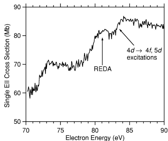
FIG. 5. Electron-impact single-ionization cross sections for the 4d \rightarrow nf, \epsilon f transitions in Xe 3+ measured with an energy resolution of 0.75 eV.
