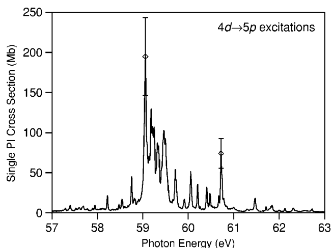
FIG. 2. Single-photoionization cross sections for the 4d \rightarrow 5p transitions in \text{Xe}^{3+} measured with an energy resolution of 20 meV. The open diamonds with error bars show the uncertainty in the absolute cross section measurements. The statistical (counting) uncertainty is as low as 0.9%.
